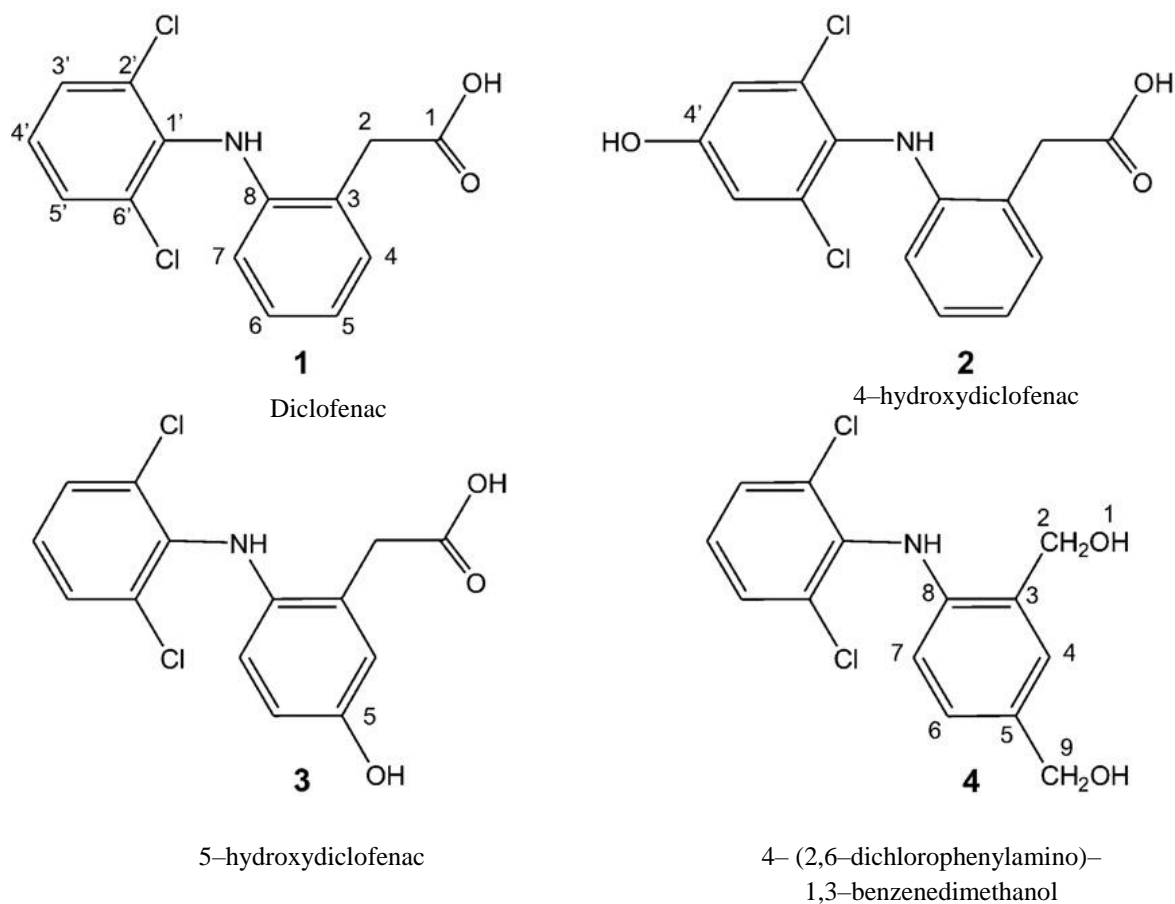
Fig. 1. Structures of diclofenac and the degradation products identified by NMR [70].
