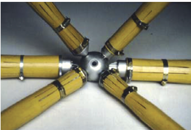
Il. 9. System Bamboutec
