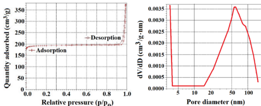
FIG. 2. \text{N}_2 adsorption-desorption isotherms (left) and pore size distribution dV/dD curves (right) of the phillipsite recrystallization product.
