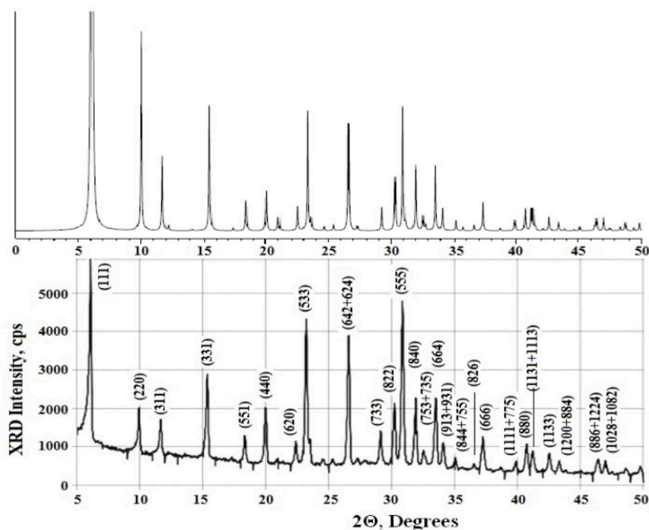
Fig. 1. Comparison of powder XRD pattern of the phillipsite recrystallization product with simulated pattern; numbers in parenthesis are Miller indices hkl .
