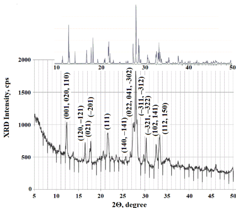
Fig. 4. Powder XRD pattern of PS with Miller indices of the most pronounced peaks compared with simulated pattern of phillipsite [K_2Ca_{1.648}(H_2O)_{12}][Si_{10.7}Al_{5.3}O_{32}] from [15].
