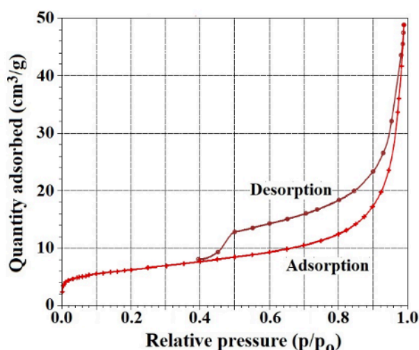
Fig. 5. N 2 adsorption-desorption isotherms of natural phillipsite.
