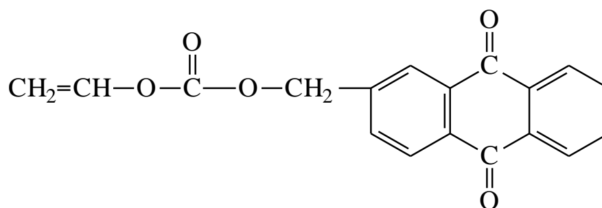
2-Vinylethoxycarbonyloxymethyl anthracinone (hydrogen abstraction type II)
