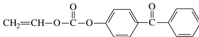
4-Benzophenylvinyl carbonate (hydrogen abstraction type II)
