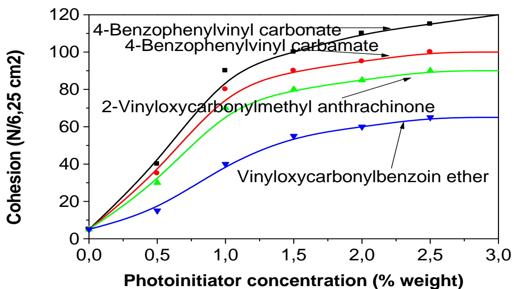
Figure 8. Shear strength of synthesized PSAs dependent on photoinitiator concentration.
