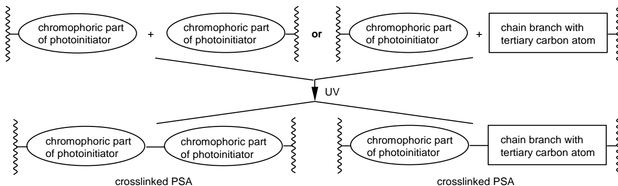
Figure 1. Photocrosslinking by using of unsaturated photoinitiators incorporated into polymer chain.
