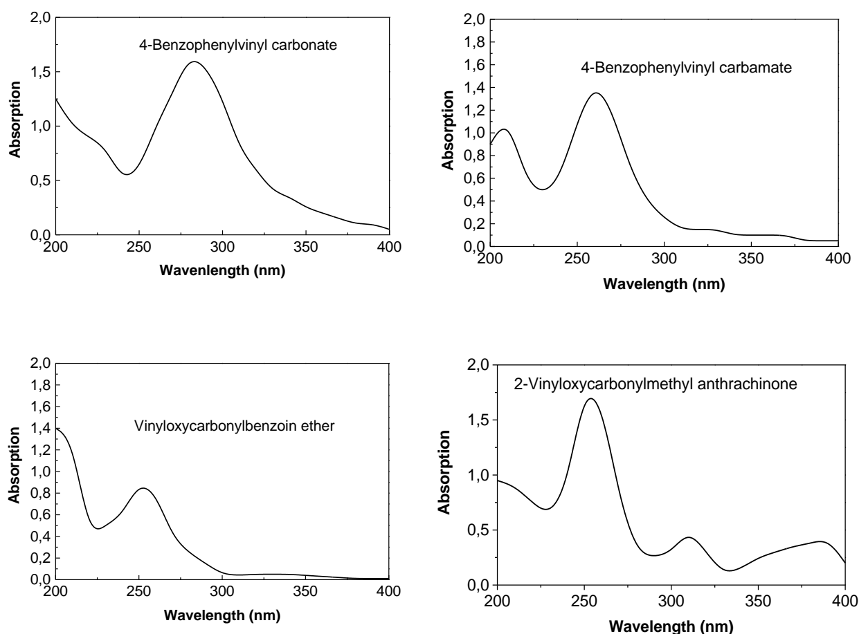
Figure 3. UV-absorption curves of investigated copolymerizable photoinitiators.
