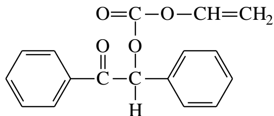
Vinylethoxycarbonylbenzoine ether ( \alpha -cleavage type I)
