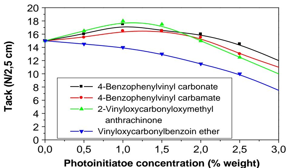
Figure 6. Tack of synthesized PSAs dependent on photoinitiator concentration.
