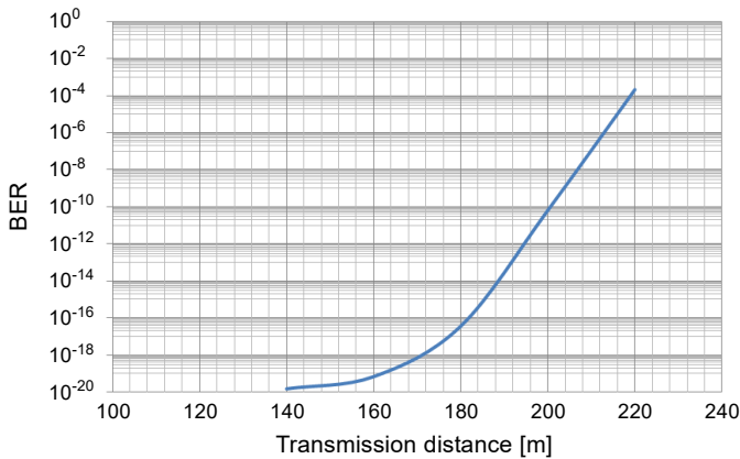
Fig. 3. Bit error rate (BER) as a function of the transmission distance of indoor VLC system.
