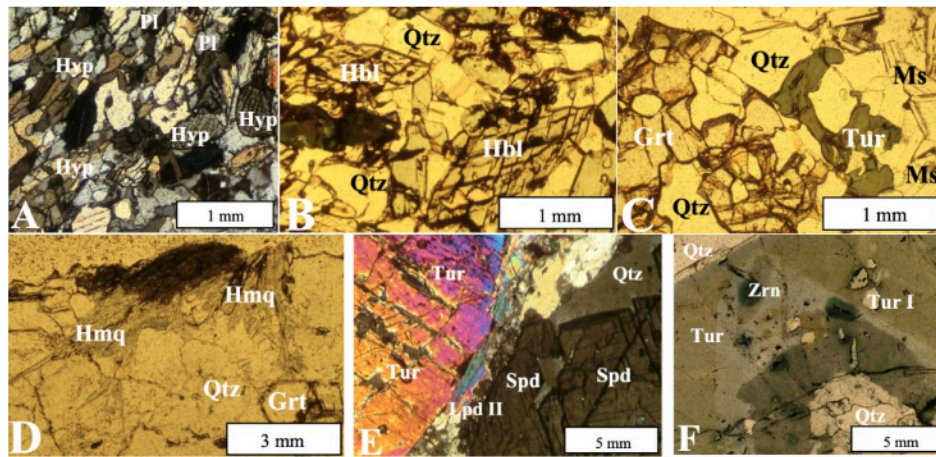
Fig. 5. Selected petrography photomicrographs of host rocks and inner pegmatite mineral intergrowths. A – metapyroxenite with hypersthene (Hyp) and plagioclase (Pl); B – amphibolitic gneisses (hornblende – Hbl, quartz – Qtz); C – metasomatic tourmaline (Tur) in a gneissic biotite-garnet (Grt) rock; D – holmsquistite (Hmq) in a metasomatic fringe from a contact between pegmatite and meta-ultramafic host; E – elbaite (Tur) / spodumene (Spd) intergrowth from inner intermediate zone with secondary lepidolite (Lpd II) and quartz (Qtz) at interface; F – early tourmaline schorl-elbaite with inherited rossmanite nucleus.
