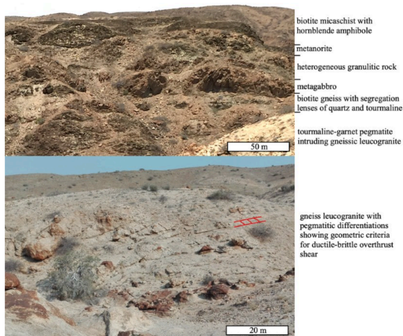
Fig. 2. Outcrop examples of host-rocks and structures spatially related to the intrusion of pegmatites.
