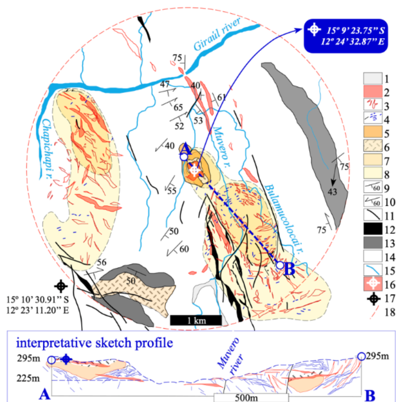
Fig. 9. Structural relations between pegmatites and host-rocks inside de original área of Giraúl IV claim. 1 - sandy placer deposits along dry rivers (“mulolas”); 2 – pegmatite bodies belonging to the LCT family (class of rare metals); 3 – outline of other, more inconspicuous, pegmatites; 4 – trajectories of the most penetrative foliations in metamorphic rocks; 5 – amphibolic and metaafic gneiss rocks including metanorites; 6 – leucogranitic breccia, with spodumene and feldspar clasts, garnet-tourmaline dissemination and some inner-fractionated small pegmatite bodies; 7 - interpretative projection to the surface of the roots system that feeds the Giraúl LCT pegmatite group; 8 – more shallower expansion of the same pegmatite system; 9 – most penetrative metamorphic foliations (measured); 10 – primitive foliation affected by a tangential overthrust transport (measured) - eventually a primitive sedimentary surface; 11 – faults; 12 – dykes of ultra-mafic rocks mainly dolerites; 13 - biotitic to amphibolic micaschists and amphibolite; 14 - undifferentiated Namibe group with micaschists, metavolcanics, gneisses and metapsamitic to metaconglomeratic layers with general granulitic to amphibolitic character; 15 – streams, creeks and rivers without surface water flow (dry rivers locally known as “mulolas”); 16 – Position of Giraúl IV landmark and respective coordinates; 17 – another set of coordinates for geographic reference; 18 – outline of the primitive area of CML claim.
