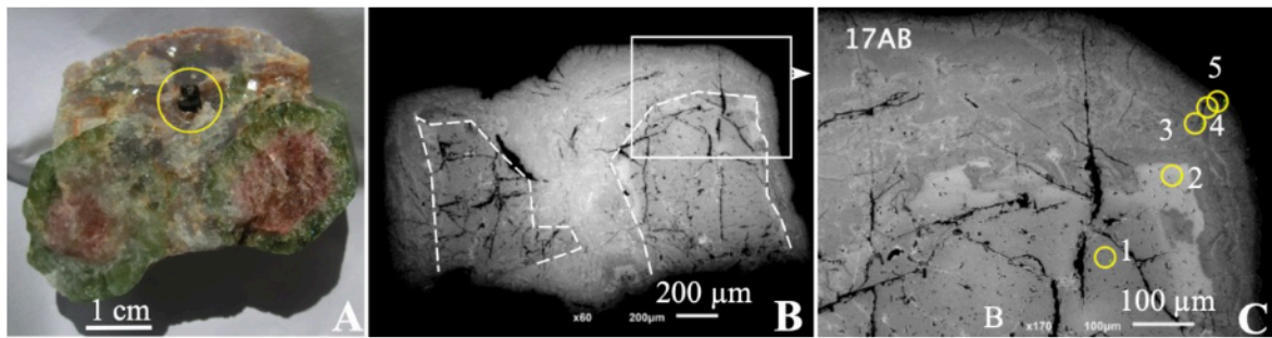
Fig. 7. Location and internal zoning of microlite in a paragenesis representative of evolutionary paroxysm in a late unit with lepidolite. A – chip sample with “water-melon” tourmaline, lepidolite and quartz where microlite crystals are located between tourmaline crystals; B – section with two coupled microlite crystals observed in scanning electron microscope (SEM) - backscattered electron mode (BE) - showing a nuclear zone related to the primary fractionation and an edge zone affected by hydrothermal alteration; C - location of the points analyzed in electron microprobe (table 1).
