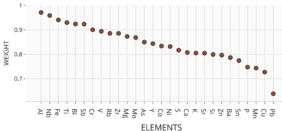
Fig. 2. Elements weights for the SOM with 6 clusters.
