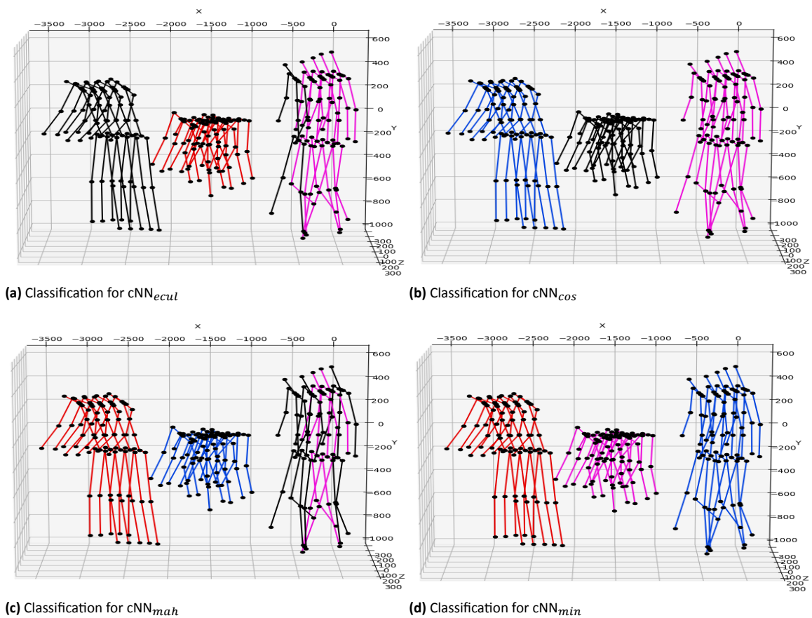
Figure 10. Stick diagrams of classification for Activity 1 (single person involved) are taken into account with four different distance metrics and configurations
