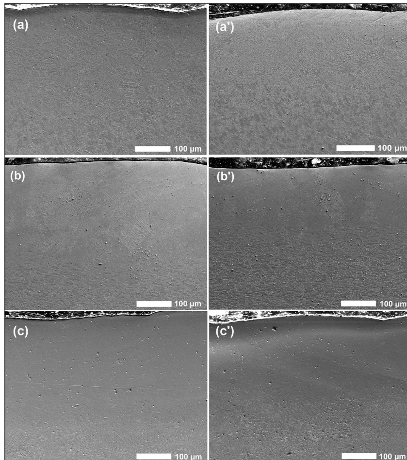
Fig. 3. Cross-sections of laser treated samples: (a) Ti_4.5, (a') Ti_3.0, (b) Ti6.4_4.5, (b') Ti6.4_3.0, (c) Ti13.13_4.5, (c') Ti13.13_3.0. (SEM)
