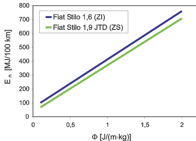
Fig. 13. Relative position of approximation straight lines (5), which have been obtained for CI and SI engine
