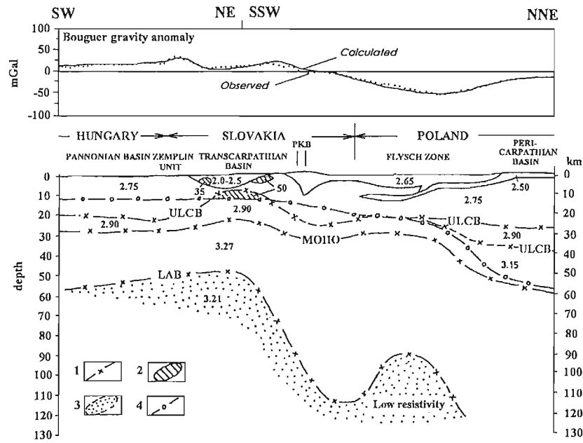
Fig. 14. Geophysical model of the lithosphere along the transect KP-X (modified according to V. Bezák et al. , 1997)
