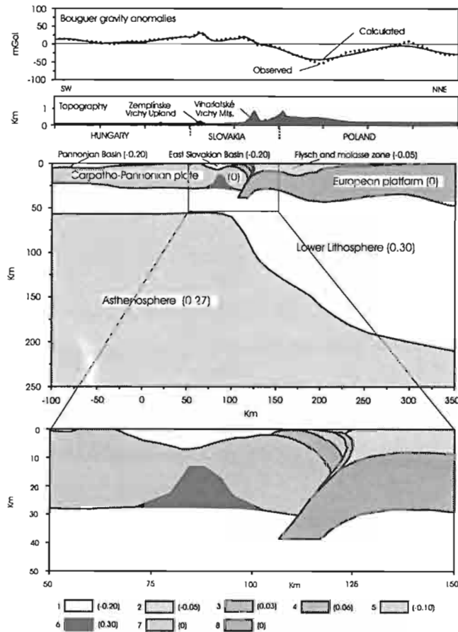
Fig. 13. Two-dimensional density model of the lithosphere along the transect KP-X
