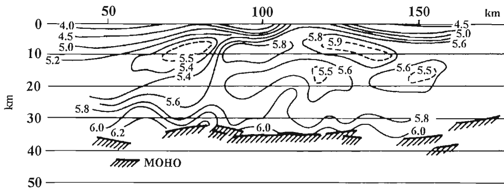
Fig. 3. Effective velocities pattern in KIII section (modified after V. Bucha, M. Blížkovský, 1994)
