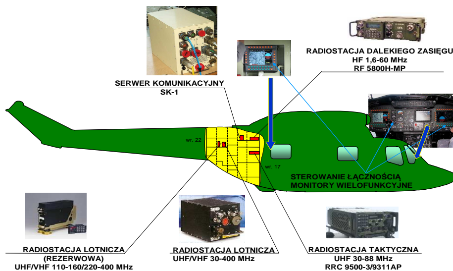
Fig. 1. The helicopter W-3PL "Głuszczyk" with components of the ITWL-developed integrated communication system ZSŁ
