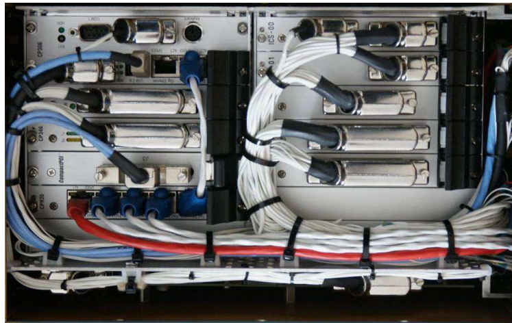
Fig. 4 The communication server of the ITWL-developed integrated communication system ZSŁ-1 built into the Mi-8, Mi-17, Mi-24, and W-3PL "Głuszc" helicopters
