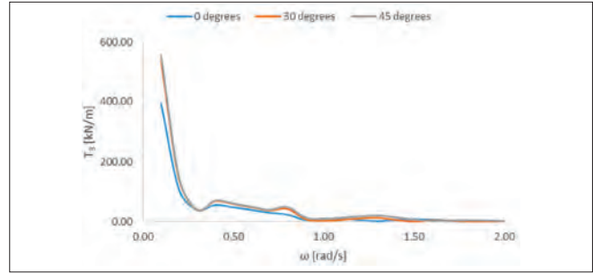
Fig. 27. Total mooring forces on the fourth mooring line
