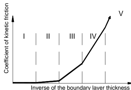
Fig. 6 Stages of passing of the porous bearing shell weakest link (oil effluent from ducts) from the fluid friction to seizure
