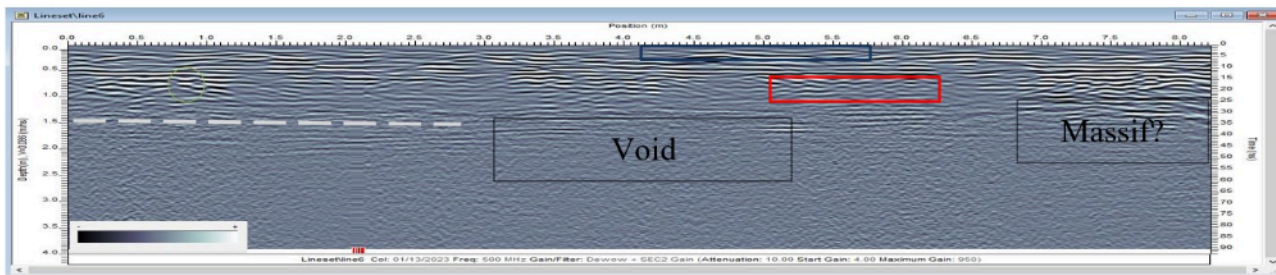
Fig. 12. Radargram Lineset 6. West acquisition. Processed.
