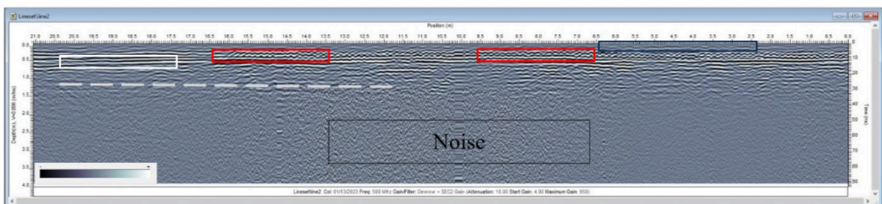
Fig. 7. Radargram Lineset 2. East acquisition. Processed.
