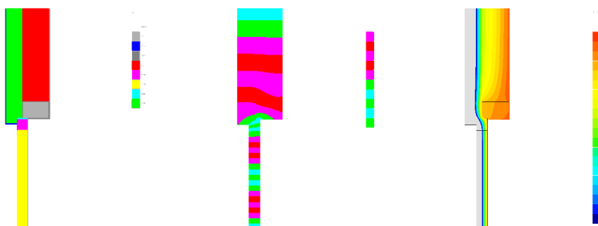
Fig. 5. Calculation model, heat flux lines (adiabates) and temperature distribution in the junction – variant III ( own research )
