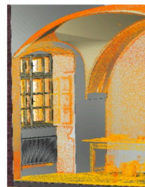
Fig. 4c. Deviation of the point cloud from the model (view)
