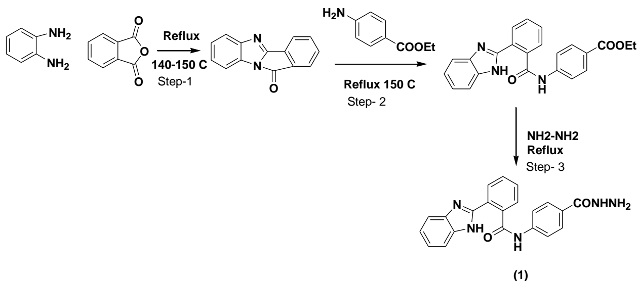
Scheme I
