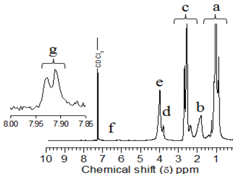
Figure 2. 1 H-NMR spectrum of P(NIPAAm 85 -co-DEAEMA 140 ) copolymers recorded in CDCl 3 at 25 °C
