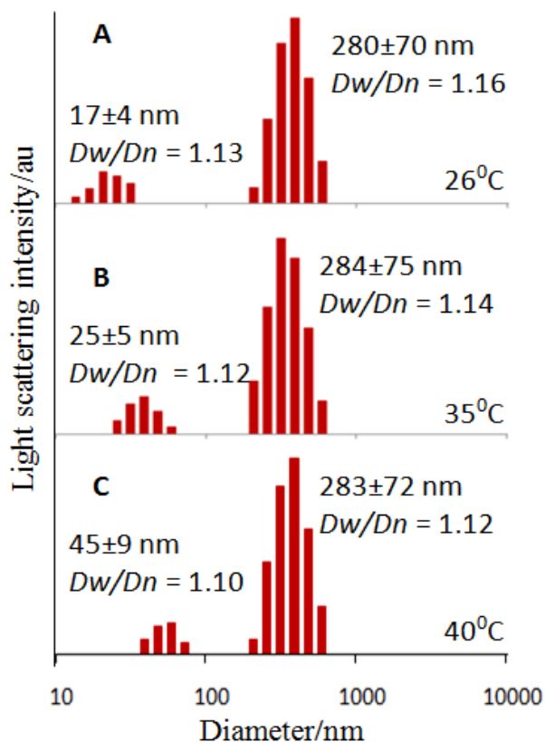
Figure 3. DLS measurement of the aqueous solution (0.0315 mM) of P(NIPAAm 85 -co-DEAEMA 140 ) copolymer at pH 4, heating rate was maintained 0.1\text{ }^\circ\text{C}/\text{min} .
