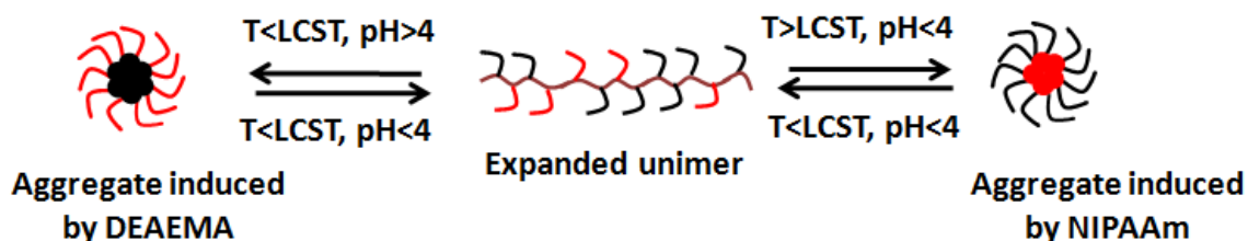
Scheme 2. Schematic presentation of aqueous dispersion phenomenon of P(NIPAAm 85 -co-DEAEMA 140 ) copolymers.
