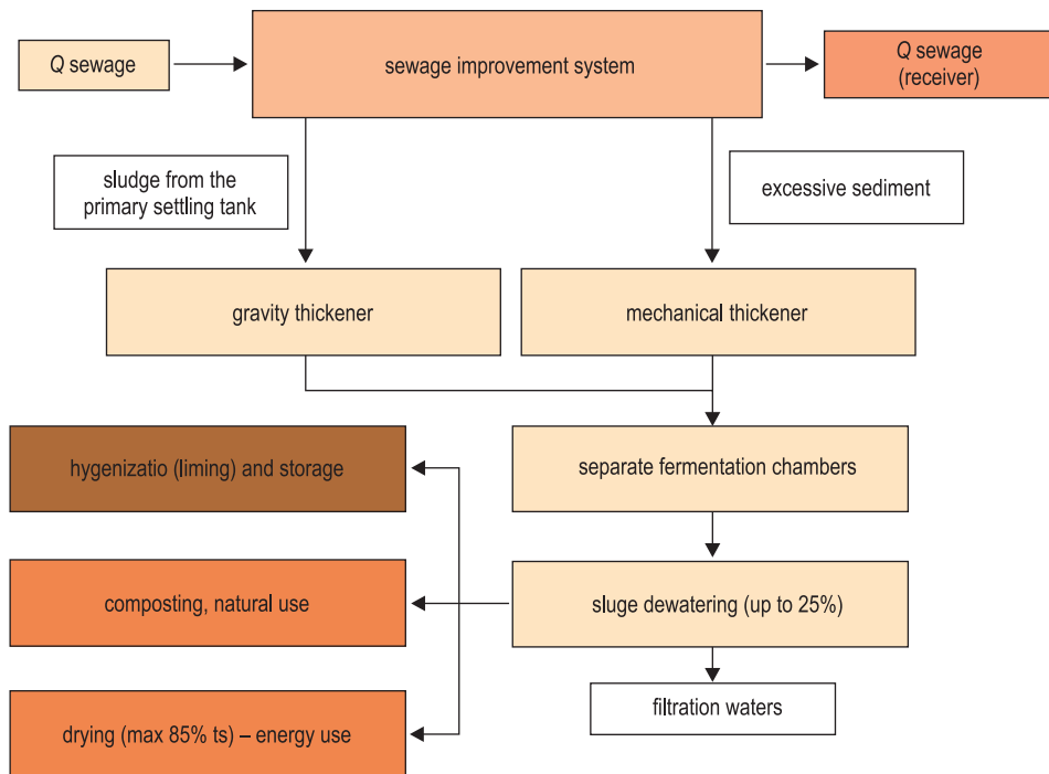
Fig. 1. Standard flow diagram of a technological line for sewage sludge treatment Source: based on GAZDA et al. (2012).
