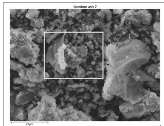
Fig. 3. Morphology of bamboo ash by SEM
