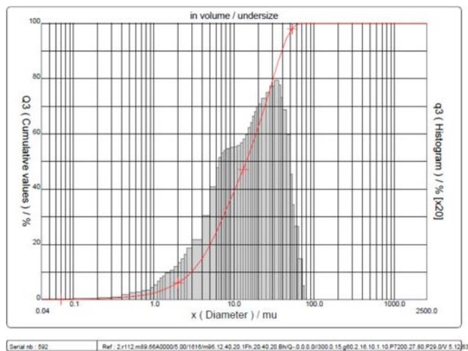
Fig. 4. Particle size distribution graph of BA
