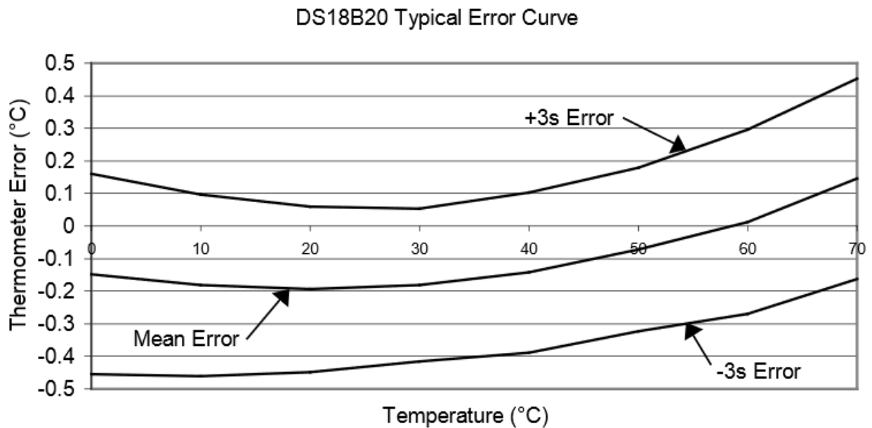
Fig. 4. The impact of temperature for the measurement error [1]
