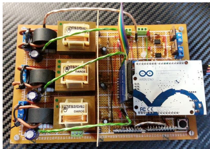
Fig. 5. Measuring system
