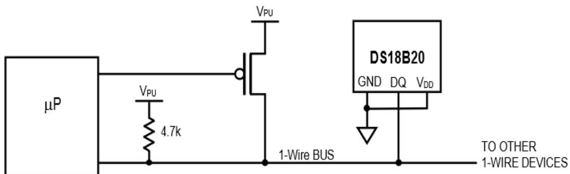
Fig. 2. Scheme of parasitic supply of sensor DS18B20 [1]
