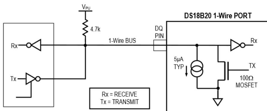
Fig. 3. Diagram of the internal structure of the transmission. [1]
