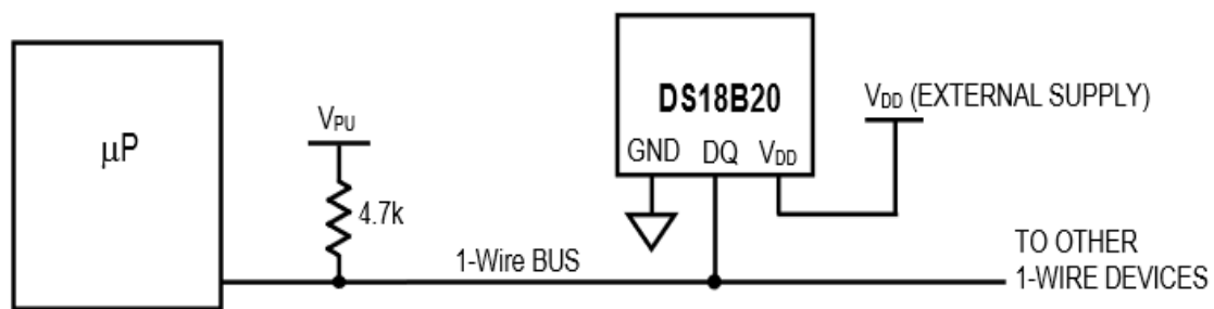
Fig. 1. Diagram of the sensor supply DS18B20 [1]
