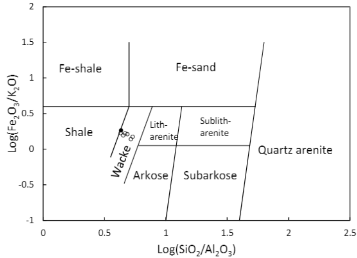
Fig. 2. Chemical classification of the Macigno sandstone samples based on \log(\text{SiO}_2/\text{Al}_2\text{O}_3) vs. \log(\text{Fe}_2\text{O}_3/\text{K}_2\text{O}) diagram of Herron, 1988 [44]. Full circle and empty circles are VE samples ( n=21 ) and MAC samples, respectively.
