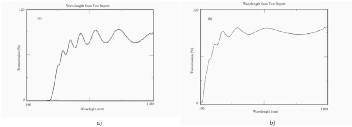
Fig. 4. a) Transmission spectra of GaN, b) Transmission spectra of AlN
