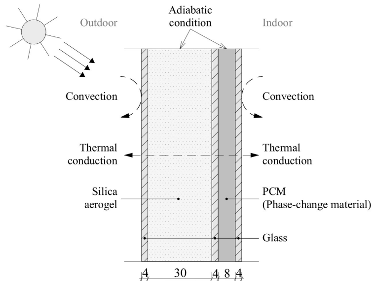
Fig. 2. A PCM and aerogel integrated window glazing system's structural configuration (according to Zhou, 2021)
