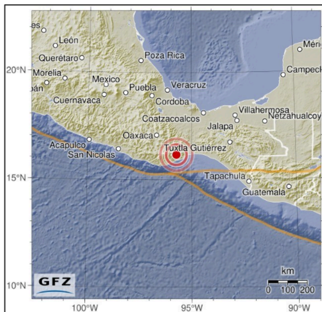
Fig. 8. Location of the earthquake from Oaxaca Mexico, 23.06.2020 (source GFZ)
