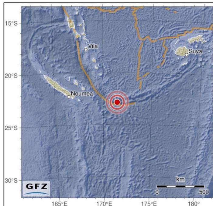
Fig. 4. Location of the earthquake from Loyalty Island, 10.02.2021 (source GFZ)
