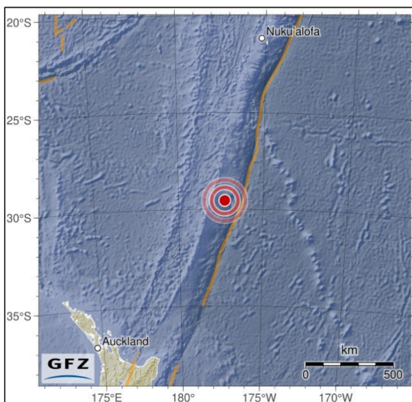
Fig. 2. Location of the earthquake from Kermadec Islands, 04.03.2021 (source GFZ)
