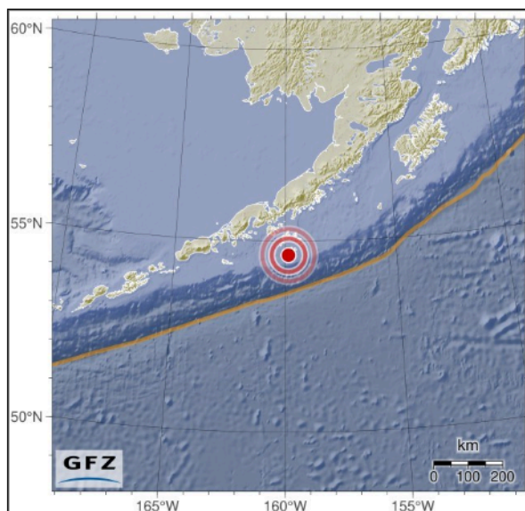
Fig. 6. Location of the earthquake from South of Alaska, 19.10.2020 (source GFZ)
