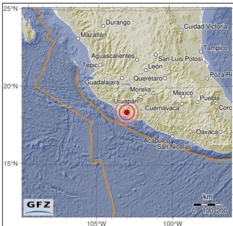
Fig. 1. Location of the earthquake from Mexico, 19.09.2022 (source GFZ)
