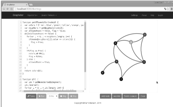
Fig. 5. Screenshot with result of running the Largest First Coloring algorithm
