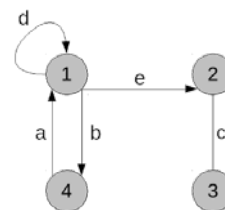
Fig. 1. Graph example: vertices – 1, 2, 3, 4; edge – c; arcs – a, b, e; loop – d
