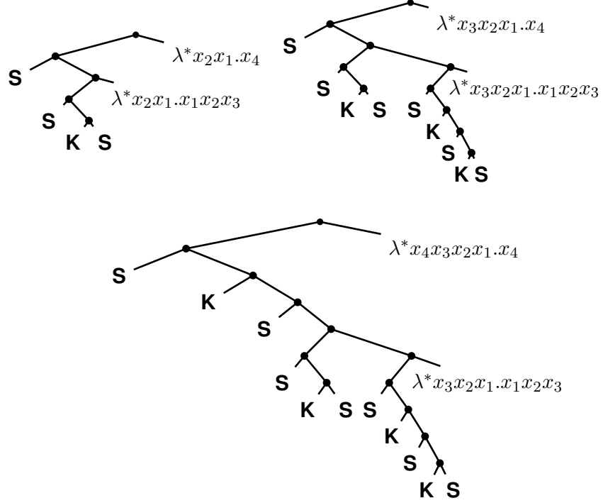
Figure 6: Three consecutive steps of the translation of the term \lambda x_4 x_3 x_2 x_1 . x_1 x_2 x_3 x_4 .
