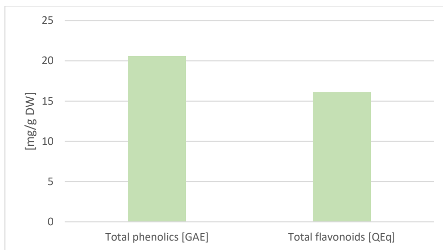
Fig. 1. Content of total phenolics and total flavonoids in P. serotina extract.
