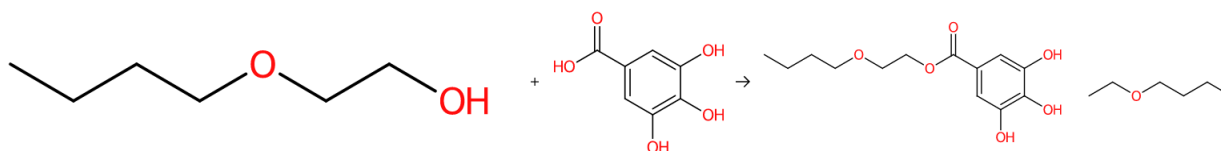
Fig. 3. Simulation of reaction between gallic acid and 2-butoxyethanol Variant I
