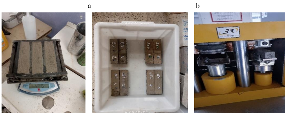
FIGURE 5. Mechanical test: a – sample preparation; b – compression strength measurement
