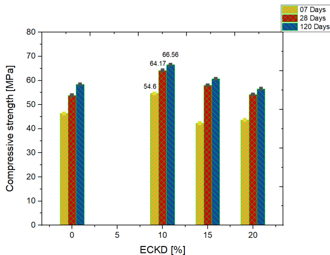
FIGURE 8. Compressive tests for several curing ages
