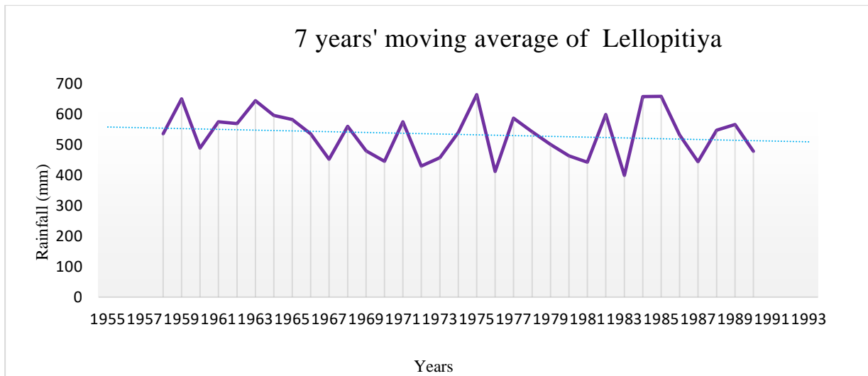
Figure 4. 7 years' moving average of Lellopitiya station
