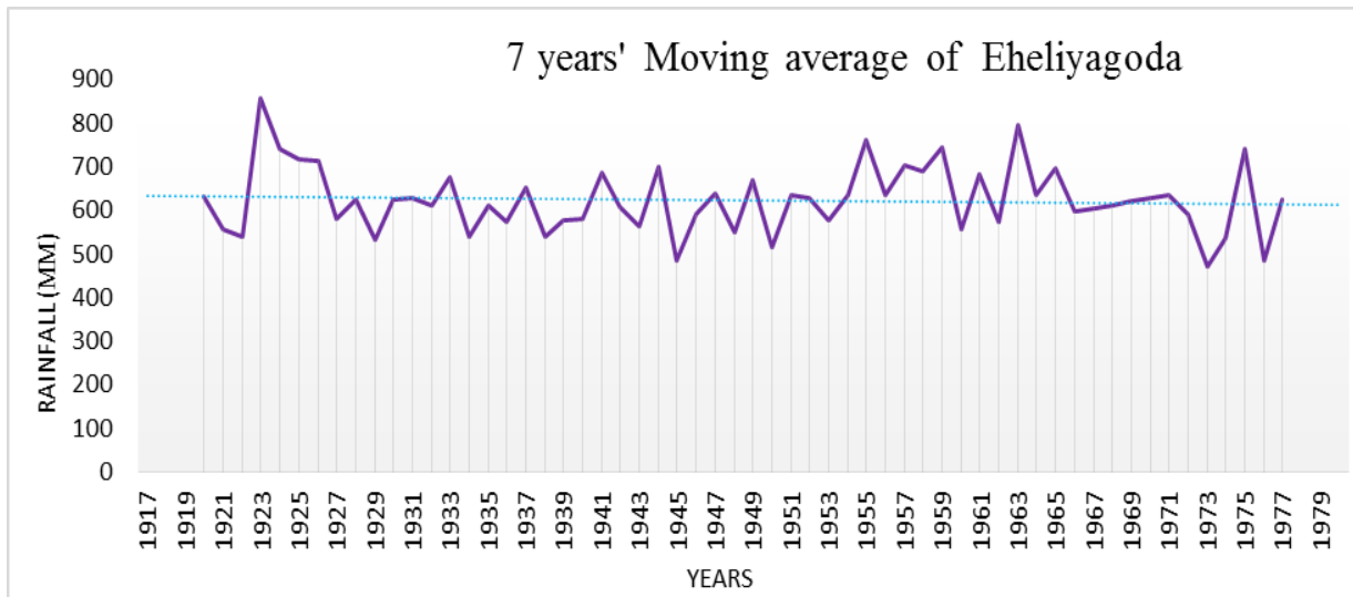
Figure 6. 7 years' moving average of Eheliyagoda station.
