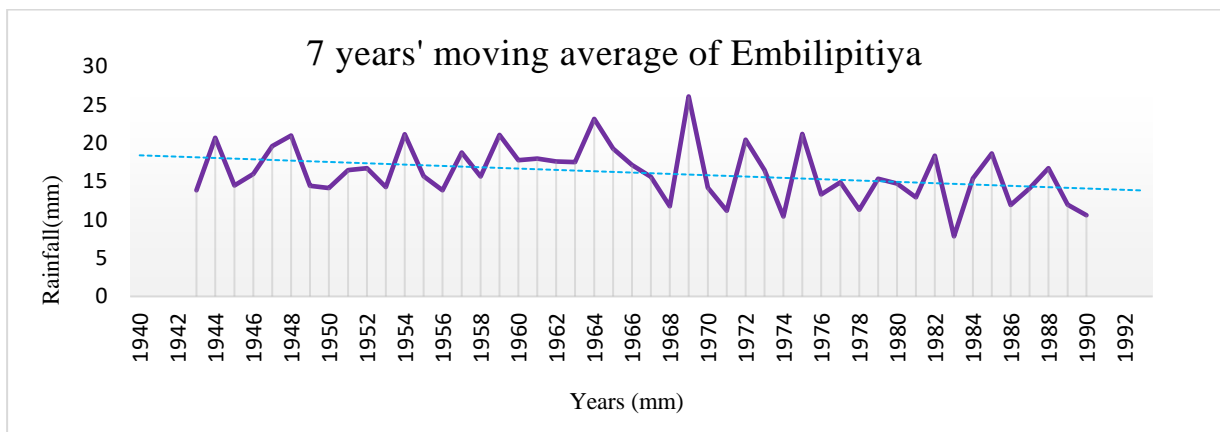
Figure 2. 7 years' moving average of Embilipitiya meteorological station
