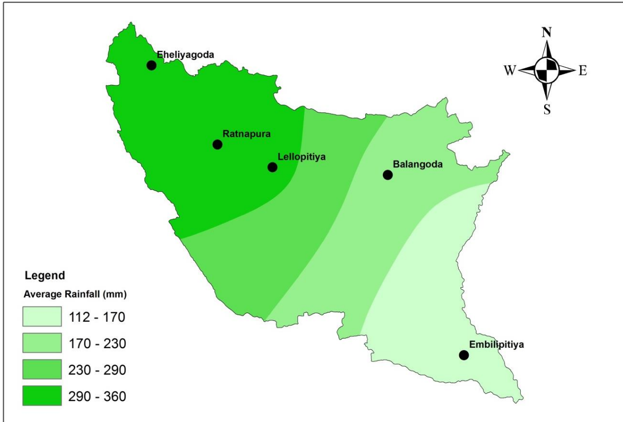
Figure 7. The annual average rainfall intensity of Ratnapura District.
