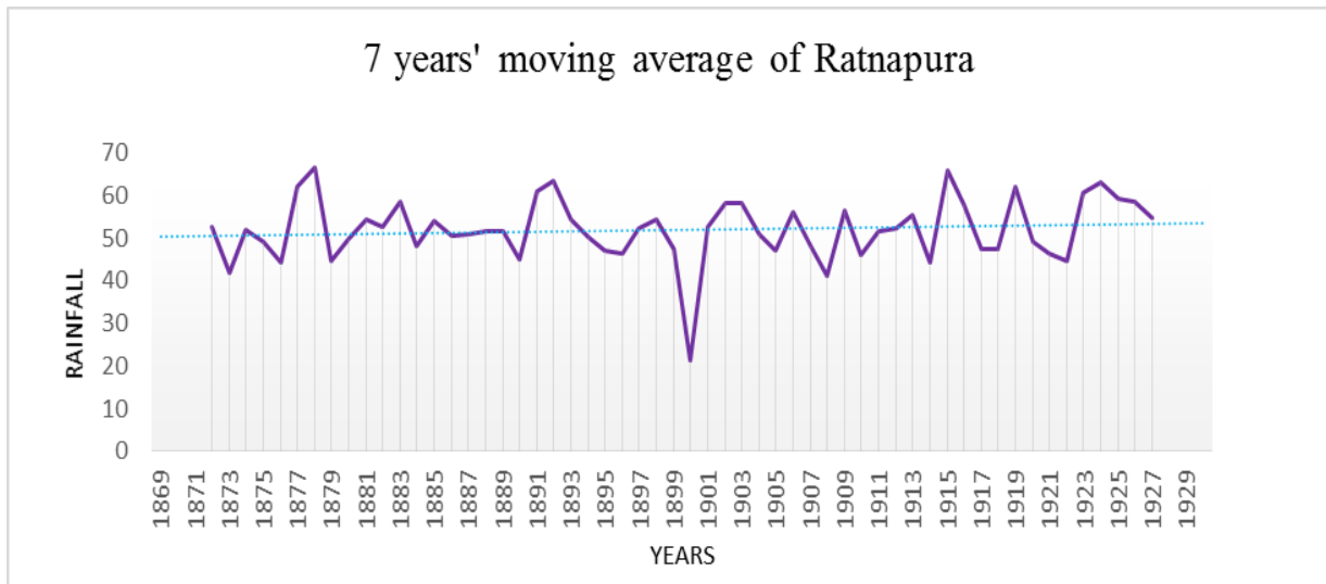
Figure 5. 7 years' moving average of Ratnapura station
