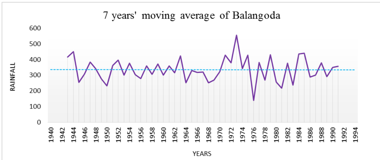
Figure 3. 7 years' moving average of Balangoda station
