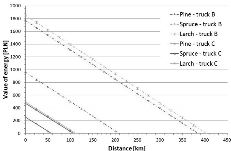
FIGURE. The balance of heat energy obtained from incineration of cones, taking into account the transport costs for a specific distance using vehicles B and C
