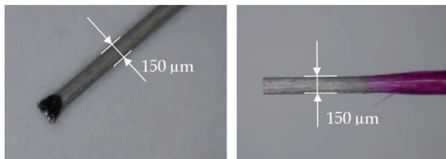
Fig. 10. Tungsten wire with a diameter of 150 \mu\text{m} , untreated with the end after manual cutting (left) and the finished end after electrochemical flattening (right)
