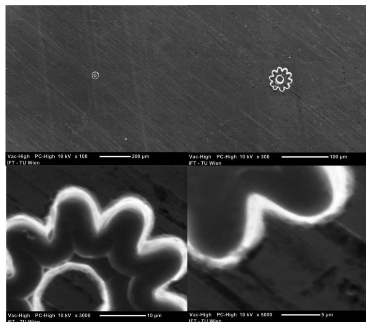
Fig. 11. Images of the microstructure, photographed with a scanning electron microscope (SEM) at different resolutions
