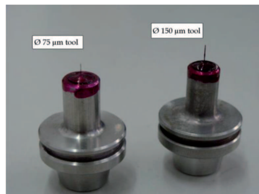
Fig. 9. Tools ready for manufacturing. The left tool has a diameter of 75 \mu\text{m} and the right tool a diameter of 150 \mu\text{m} , both with Lacomit layer
