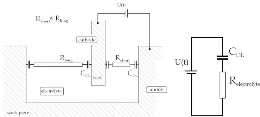
Fig. 7. Schematic illustration of the electrochemical double layers as capacitors and the electrolyte as electrical resistor between tool and work piece (left) and the equivalent circuit diagram (right) with U(t) as energy source, C_{DL} as capacitance of the double layers and R_{electrolyte} as the ohmic resistor of the electrolyte
