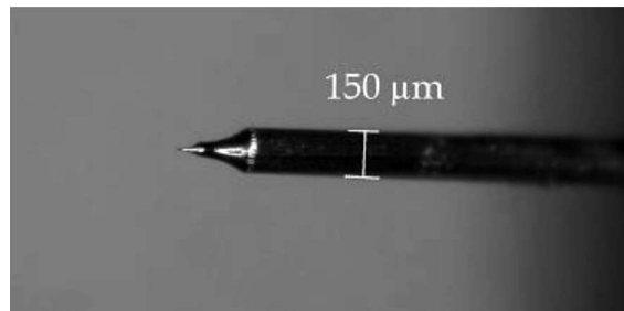
Fig. 12. Image of the tool to produce the micro injection mould with a top of D < 5\ \mu\text{m}
