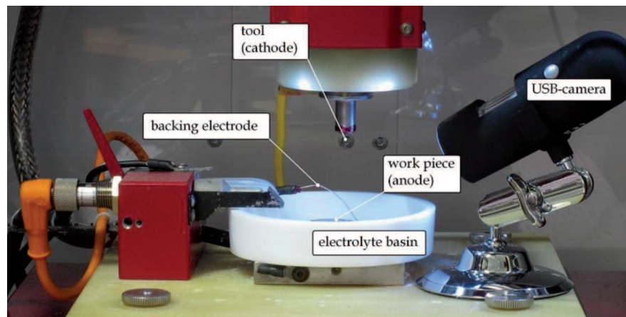
Fig. 5. View inside the electrochemical machine with all important parts for the manufacturing process labelled
