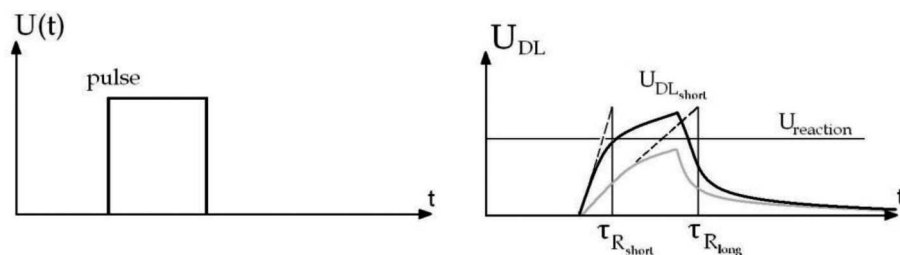
Fig. 8. Applied voltage pulse (left) and time-variable voltage curve in the electrochemical double layer (right)
