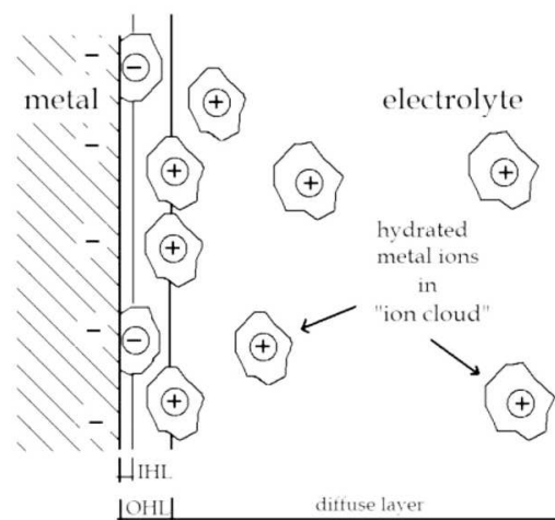
Fig. 6. Simplified Stern-Graham-Model of the electrochemical double layer [2]
