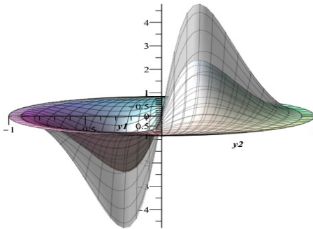
Fig. 3. Graphs of the given and calculated final functions, \gamma = 0.026
