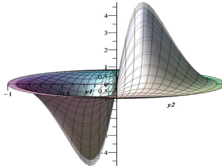
Fig. 4. Graphs of the given and calculated final functions, \gamma = 0.014
