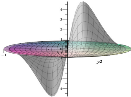
Fig. 1. Graphs of the given and calculated final functions, \gamma = 1
