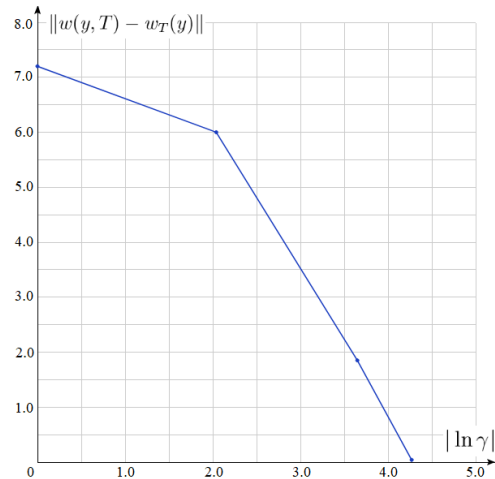
Fig. 5. Graph of the values of the minimized functional (excluding the regularizing term)
