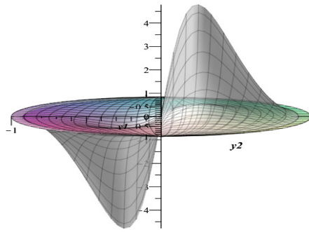
Fig. 2. Graphs of the given and calculated final functions, \gamma = 0.13
