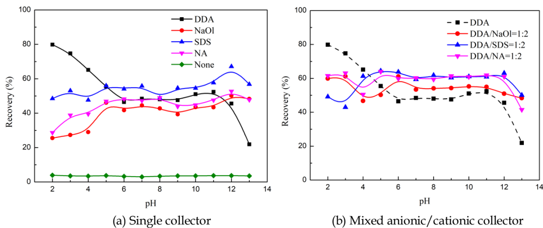
Fig. 2. The effect of pH on the recovery of muscovite under the condition of a collector concentration of 2.0 \times 10^{-4} mol/L
