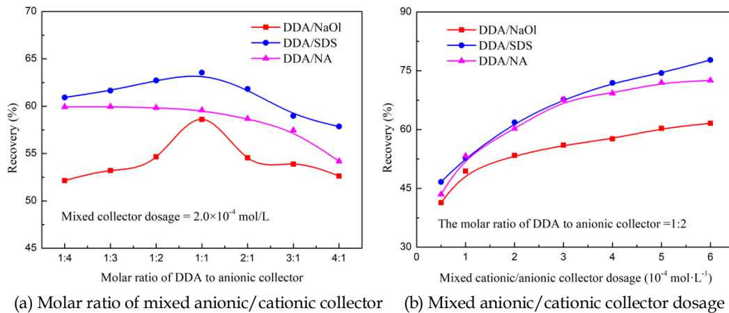
Fig. 3. The relationship between the recovery of muscovite and the mixed anionic/cationic collector at pH=7
