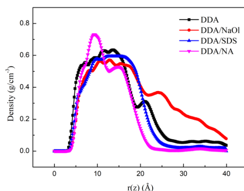
Fig. 10. The calculated density distribution of carbon atoms on the muscovite (001) surface in different flotation systems
