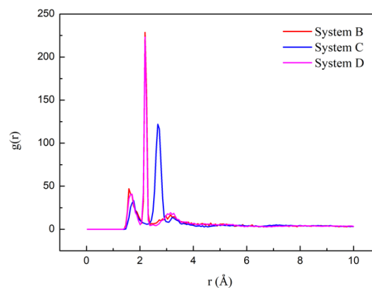
Fig. 7. The calculated RDF for the hydrogen atoms in the amino groups and the oxygen atoms in the anionic collectors in different flotation systems
