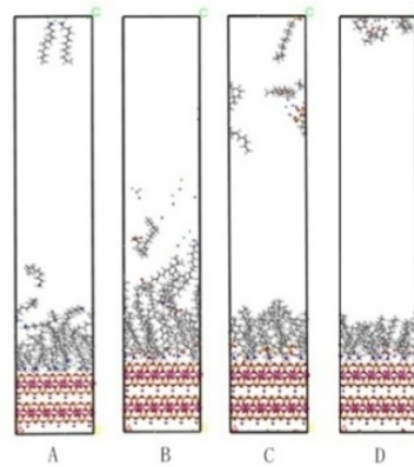
Fig. 5. The stable configuration of different collectors adsorbed on the muscovite (001) surface (the blue, red and yellow spheres represent nitrogen, oxygen and silicon respectively; the water molecule have been hidden)
