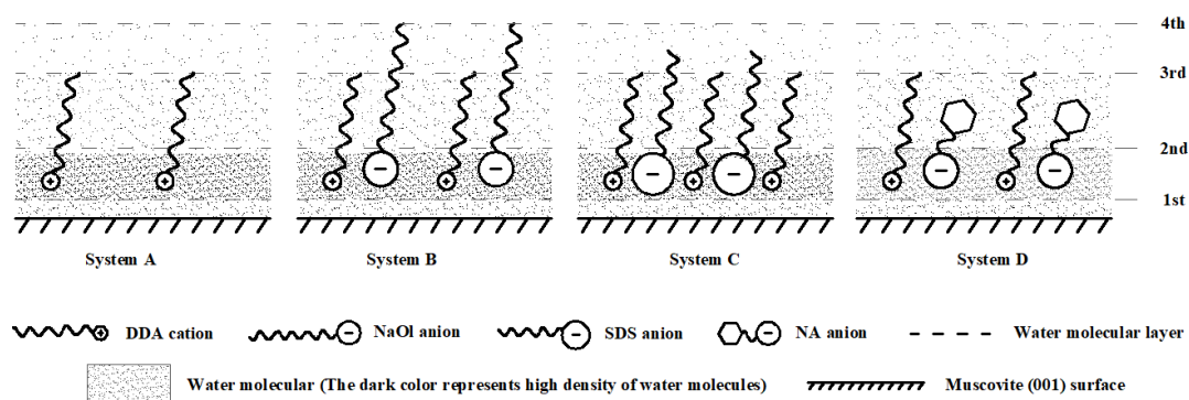
Fig. 11. The adsorption mechanism of different mixed anionic/cationic collectors on the muscovite (001) surface
