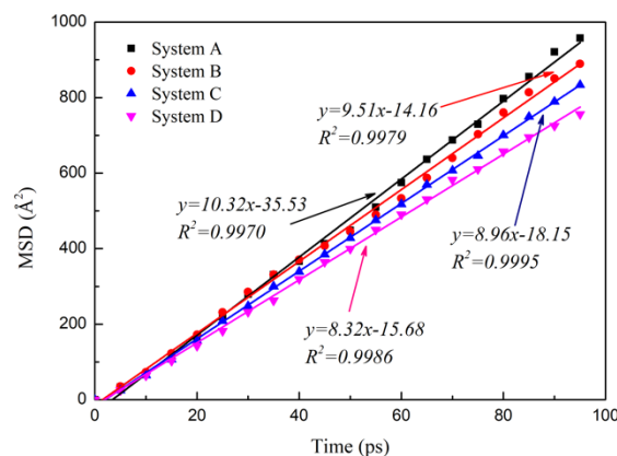
Fig. 9. The calculated MSD curves of water molecules on the muscovite (001) surface for 100 ps after dynamic equilibrium in different flotation systems
