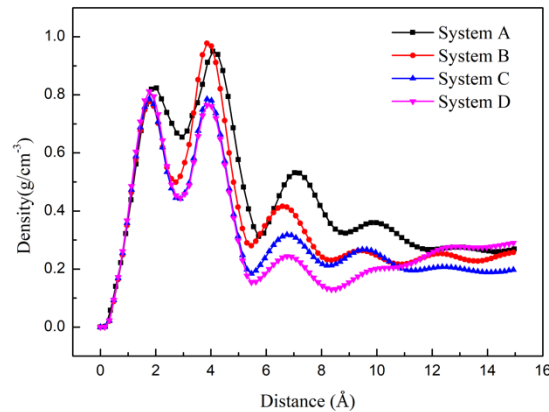
Fig. 8. The calculated density distribution of O_{\text{water}} atoms on the muscovite (001) surface in different flotation systems
