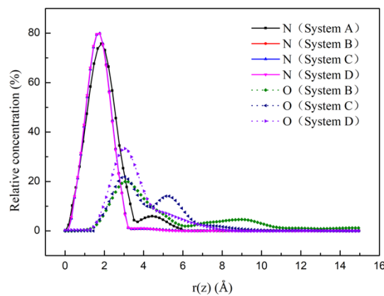
Fig. 6. The calculated distribution function of nitrogen atoms in DDA cations and hydroxyl oxygen atoms in anionic collectors along the Z-axis in different flotation systems
