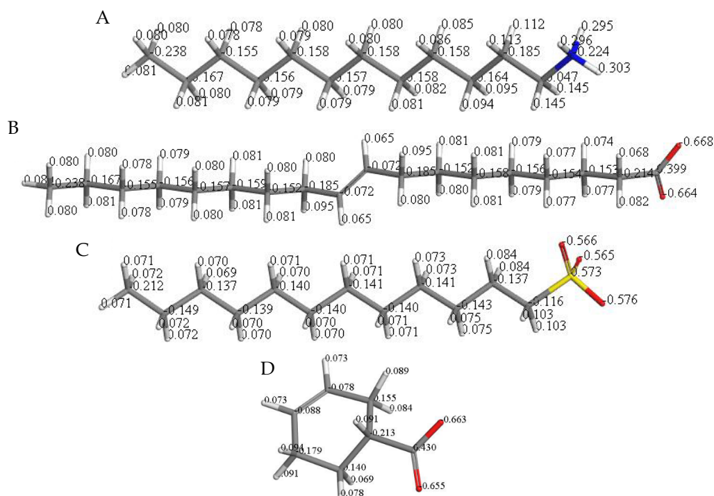
Fig. 1. The Mulliken populations of the optimized collector molecules (A: DDA cation, B: NaOl anion, C: SDS anion and D: NA anion) in an aqueous solution (the white, gray, blue, yellow and red sticks represent hydrogen, carbon, nitrogen, sulfur and oxygen, respectively)
