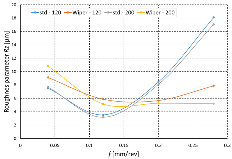
Fig. 4. The influence of the feed f on the values of the roughness parameter Rz of the machined surface (workpiece material - XCrNiNb18-9)
