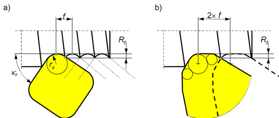
Fig. 1. Scheme of theoretical roughness formation during turning with cutting inserts with a corner: a) conventional, b) Wiper [10]
