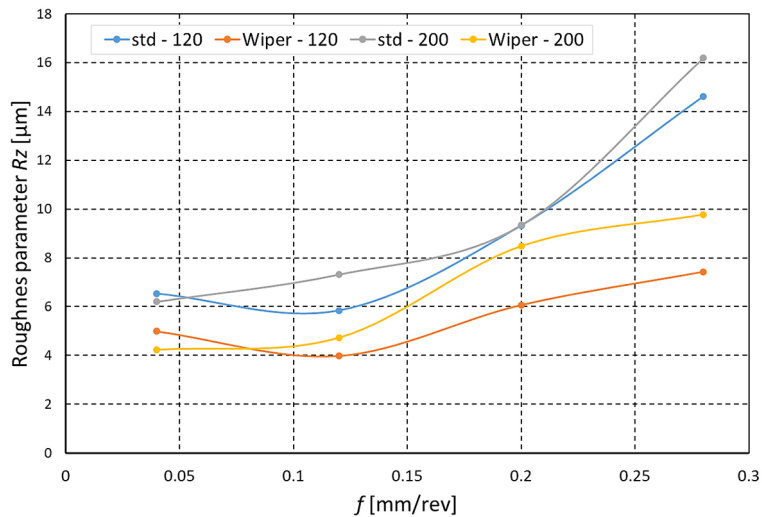
Fig. 6. The influence of the feed f on the values of the roughness parameter R_z of the machined surface (workpiece material - 14NiCr14)
