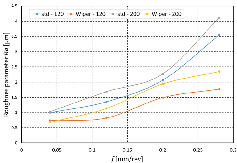
Fig. 5. The influence of the feed f on the values of the roughness parameter Ra of the machined surface (workpiece material - 14NiCr14)
