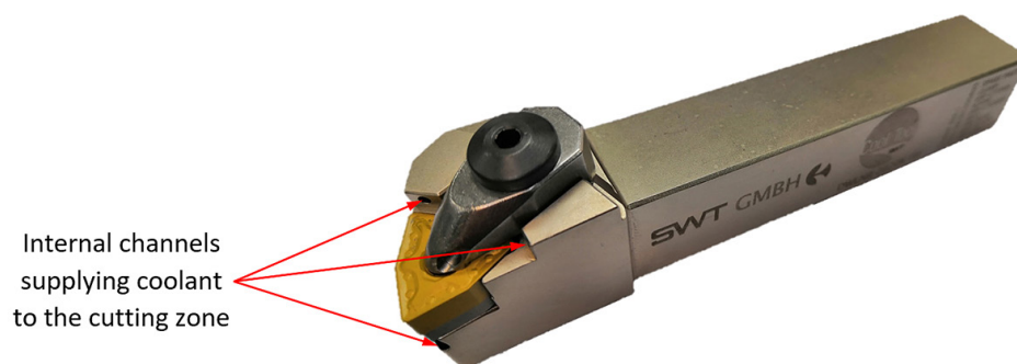
Fig. 2. The tool used in the research
