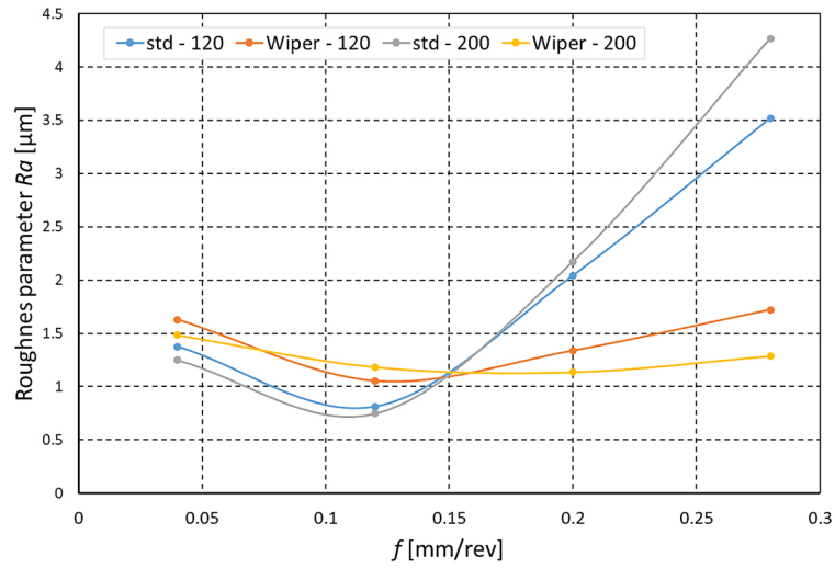
Fig. 3. The influence of the feed f on the values of the roughness parameter Ra of the machined surface (workpiece material - XCrNiNb18-9)
