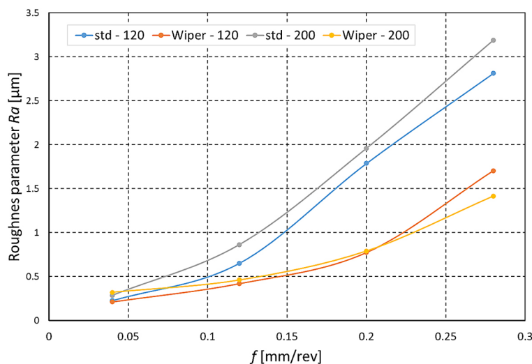
Fig. 7. The influence of the feed f on the values of the R_a roughness parameter of the machined surface (workpiece material - A356)
