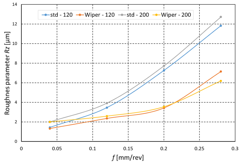
Fig. 8. The influence of the feed f on the values of the Rz roughness parameter of the machined surface (workpiece material - A356)
