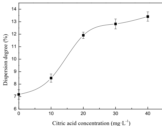
Fig. 4. Dispersion degree of the mixture (siderite-hematite) as a function of citric acid concentration
