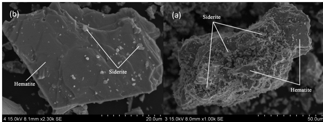
Fig. 3. SEM images of mineral particles in the foam product of the mixtures flotation: (a) without citric acid; (b) with citric acid at a concentration of 20 mg/dm 3
