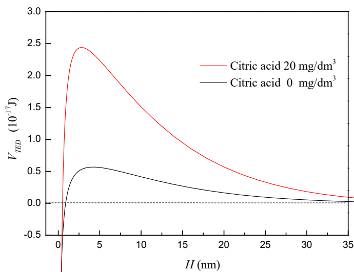
Fig. 8. Total interaction energy between siderite and hematite particles in the presence and absence of citric acid
