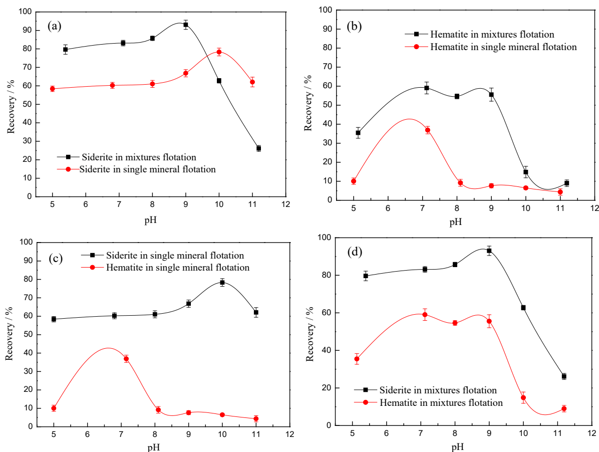
Fig. 1. Recovery as a function of pH value: siderite (a) and hematite (b) in the single mineral flotation and the mixtures flotation; siderite and hematite in the single mineral flotation (c) and the mixtures flotation (d) (sodium oleate concentration: 150 mg/dm 3 ; corn starch concentration: 20 mg/dm 3 , the single mineral sample: 2.0 g of -18 \mu m siderite or -74 \mu m hematite; the mixtures sample: 0.4 g of -18 \mu m siderite and 2.0 g of -74 \mu m hematite)
