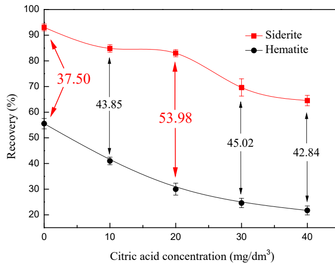
Fig. 2. Recoveries of siderite and hematite in the mixtures flotation as a function of citric acid concentration (sodium oleate concentration: 150 mg/dm 3 ; corn starch concentration: 20 mg/dm 3 ; pH: 9.0)
