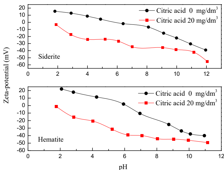
Fig. 6. Zeta potentials of siderite and hematite as a function of pH value in the presence and absence of citric acid
