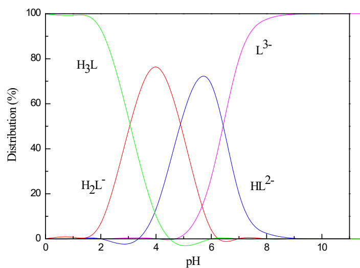
Fig. 7. Species distribution diagram of citric acid 1.04 \times 10^{-4} mol/dm 3 as a function of pH value (Hu et al., 1998)
