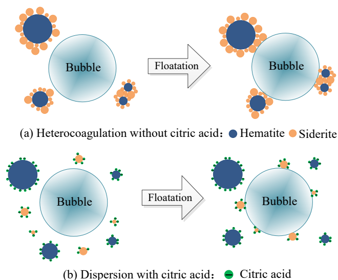
Fig. 9. Eliminating coating and coagulation effects of particles in flotation due to the dispersing effect of citric acid
