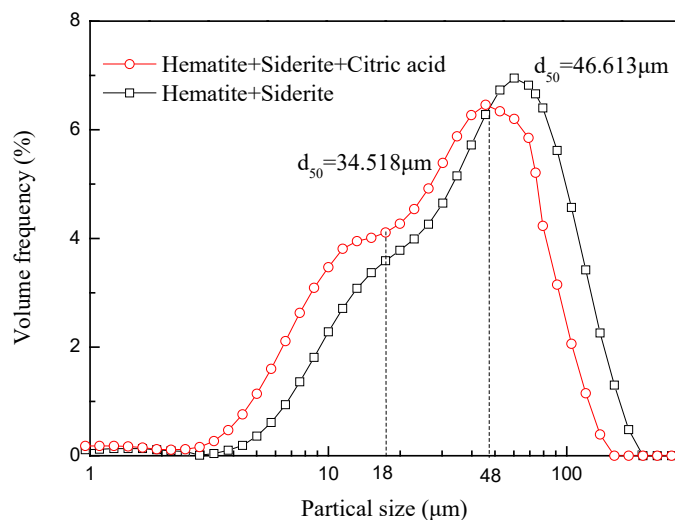
Fig. 5. The volume size distributions of the particles in the pulp (0.4 g of -18 \mu\text{m} siderite and 2.0 g of -74 \mu\text{m} hematite)
