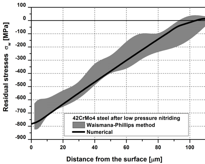
Fig. 9. Distribution of residual stresses in 42CrMo4 steel after low pressure nitriding
