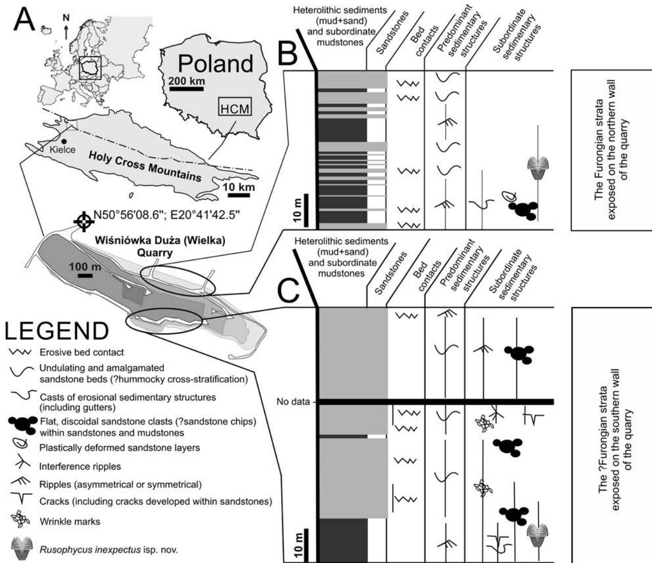
Fig. 1. Location of Wiśniówka Duża (“Wielka” in older literature) Quarry and general profiles of strata, exposed on northern and southern walls. A. Location of Wiśniówka Duża Quarry. B. The general profile of northern wall. C. General profile of southern wall. A question mark for the Furongian age in description of southern wall profile comes from the lack of direct body index fossils for this interval (see text).
