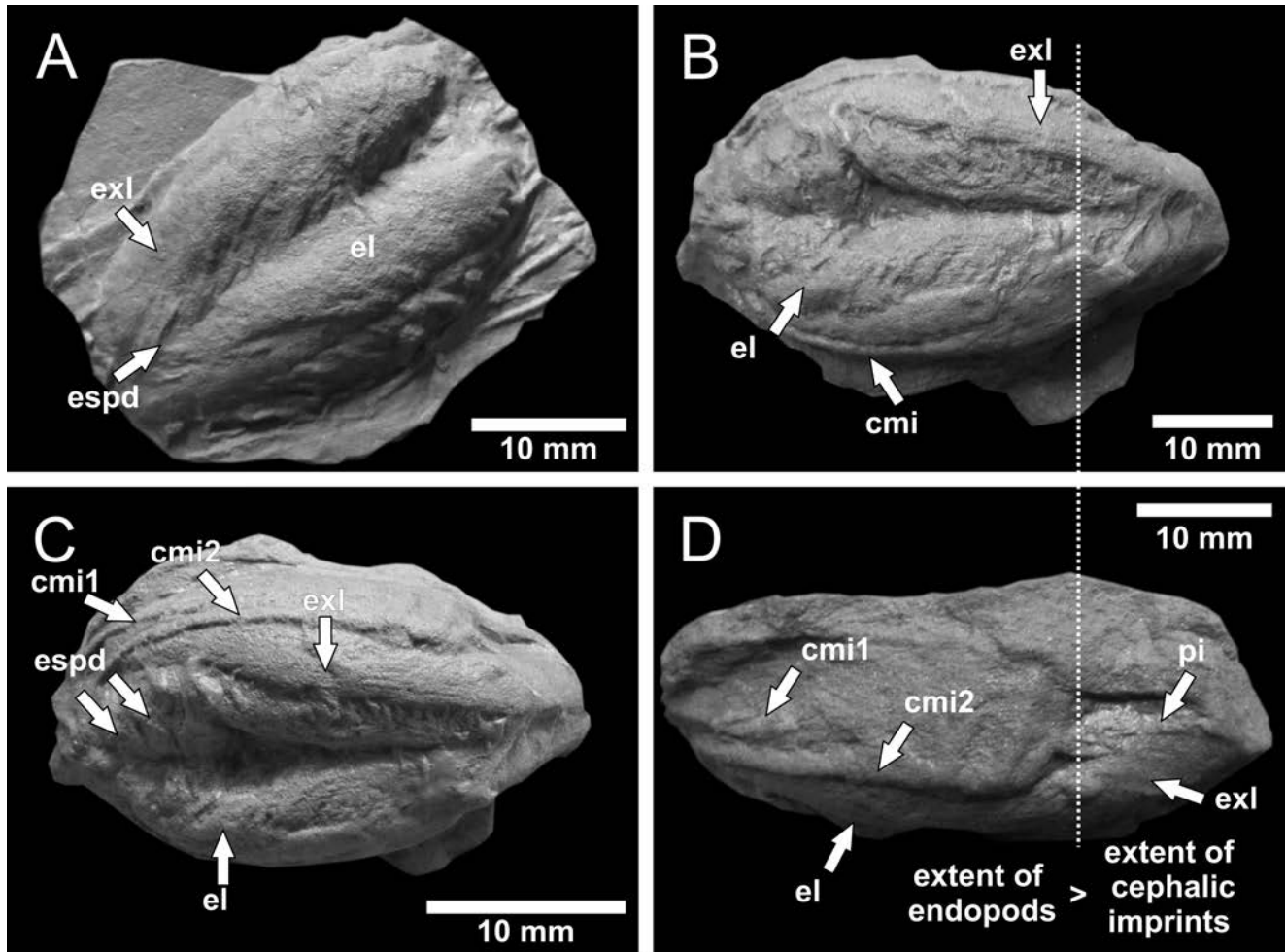
Fig. 4. Rusophycus arizonensis (Seilacher) ( Cruziana arizonensis Seilacher, 1970) displaying trilobite-like pattern of tagmosis. A. Trace fossils with all endopodal scratches directed posteriorly; GPIT/IC/00149. B–D. Well preserved trace fossils with cephalic imprints (various views of the same specimen; GPIT/IC/00150). Note that endopodal scratches extend beyond rear margin of cephalic imprint (B and D: shown by dashed line). Symbols used: see caption of Figure 2.
