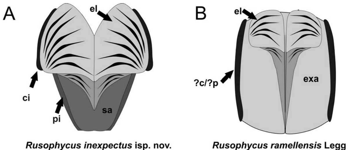
Fig. 5. Comparison of Rusophycus inexpectus isp. nov. and Rusophycus ramellensis Legg: schematic drawing. Drawing in B is based on specimen, illustrated in Fig. 3D. Symbols used: see caption of Figure 2.
