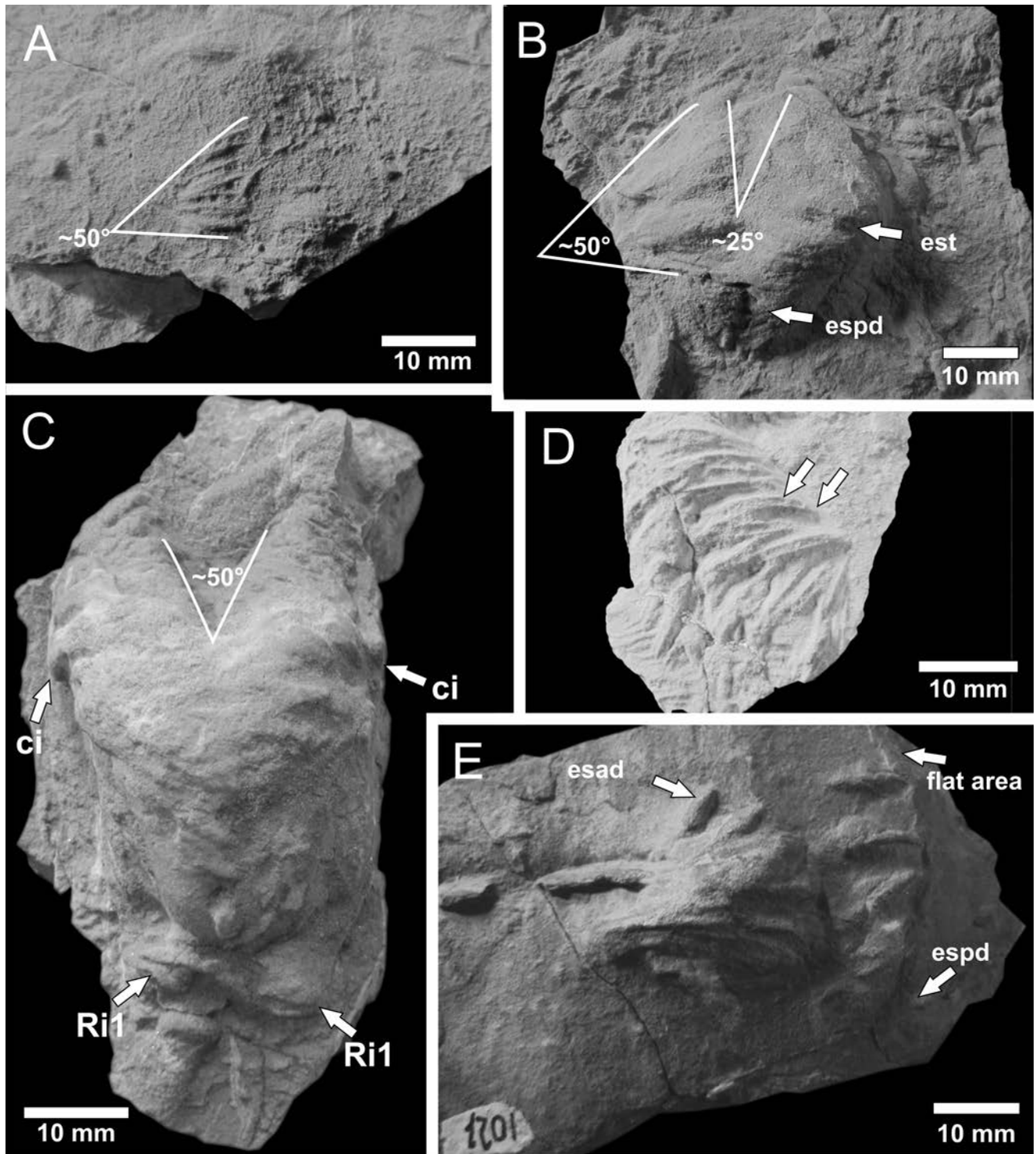
Fig. 2. Rusophycus inexpectus isp. nov. from the Wiśniówka Sandstone Formation. Symbols used on figures: esad – endopodal scratches anteriorly directed, espd – endopodal scratches posteriorly directed, esapd – endopodal scratches anteriorly to posteriorly directed, esatd – endopodal scratches anteriorly directed to transverse, est endopodal scratches transverse, ci – cephalon imprint, Ri1 – first Rusophycus inexpectus , ?c/?p – ?cephalic/?pleural imprints, el – endopodal lobe, sa – smooth area, exa – exopodal area, pi – pleurae imprints, cmi1, 2, 3 – cephalic margin imprint number 1, 2, 3. A. Shallow expression of the trace fossil (ZPAL Tf. 4/1335). B. Deeper expression of the trace fossil (typical “moustache-like” pattern of scratches; ZPAL Tf. 4/912). C. Full version of the trace fossil (ZPAL Tf. 4/1329), note the shallow version of the trace fossil, located close to the posterior margin of this specimen (Ri1). D, E. Two shallow expressions of the trace fossil (D: ZPAL Tf. 4/1331; E: ZPAL Tf. 4/1023).
