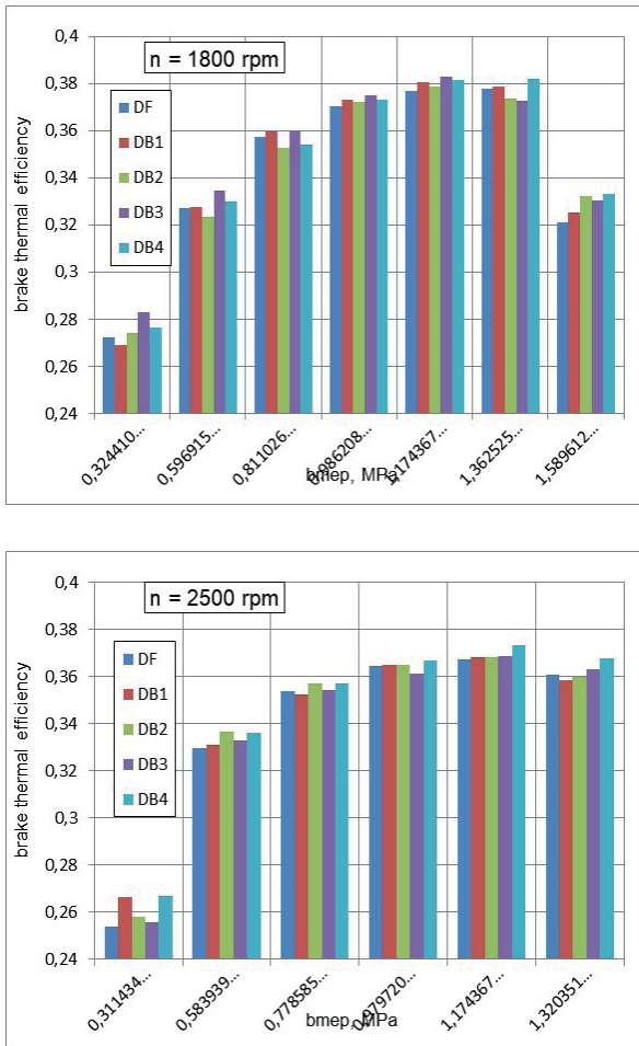
Fig. 7. The brake thermal efficiency (bte) as a function of engine load (bmep) when using various diesel-n-butanol fuel blends at speeds of 1800 and 2500 rpm.
