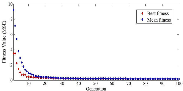
Fig. 4. Best fitness convergence of the problem
