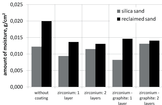
Fig. 5. Amount of moisture sorped from surroundings during 12 hours
