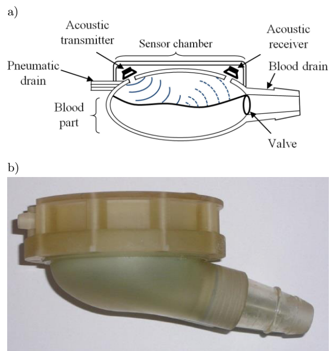
Fig. 5. Idea of the POLVAD-EXT model equipped with an additional sensor chamber (a) and the practical realization (b).
