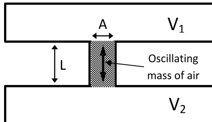
Fig. 2. Helmholtz's resonator.
