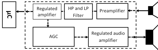
Fig. 6. Block diagram of the final version of the measurement system.
