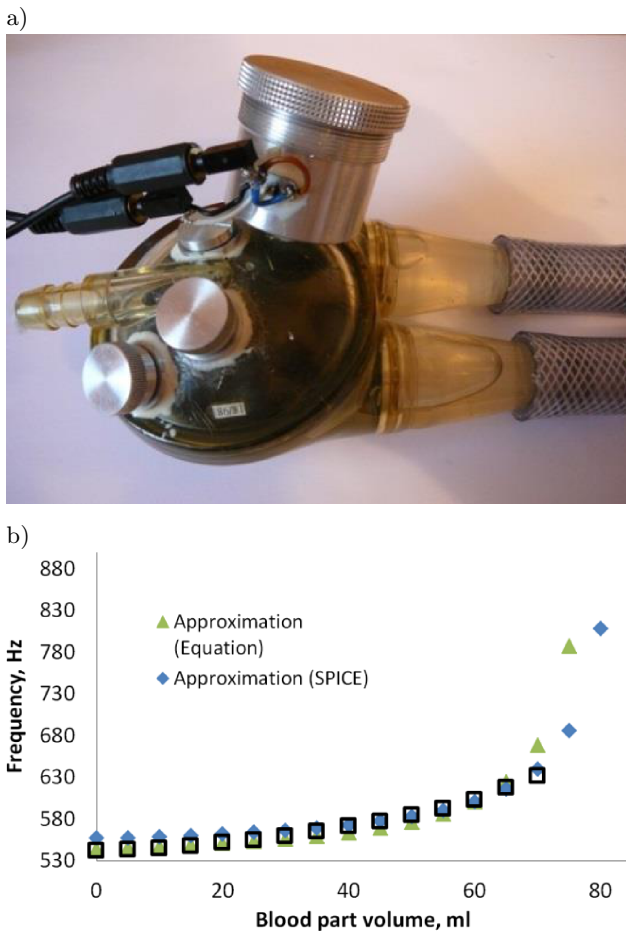
Fig. 4. POLVAD-MEV with the sensor part (a) and theoretic and practical results of the measurements (KONIECZNY et al. , 2009; 2011).
