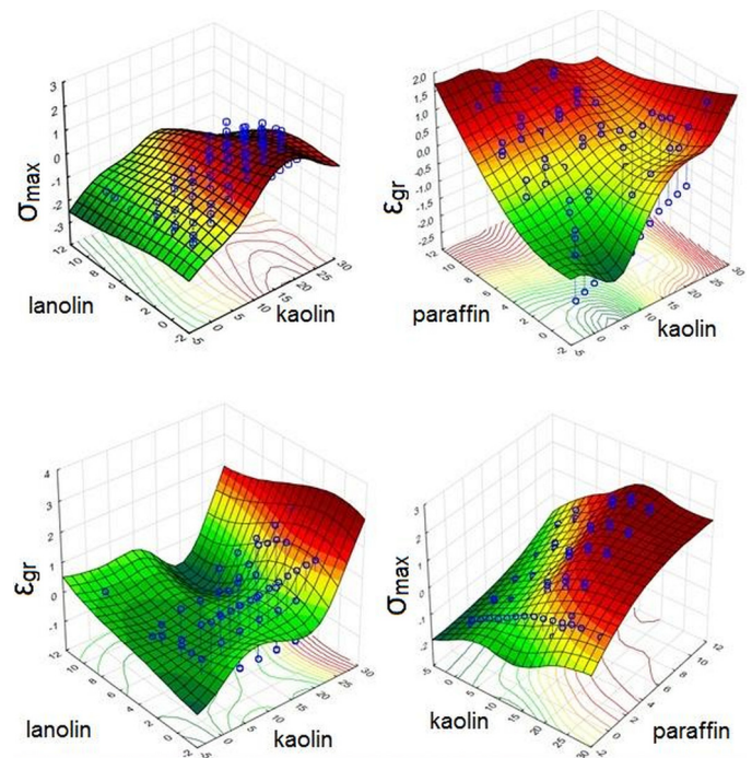
Fig. 7. Compilation of 3-D scatter diagrams showing the total effect of the selected components on the particular properties
