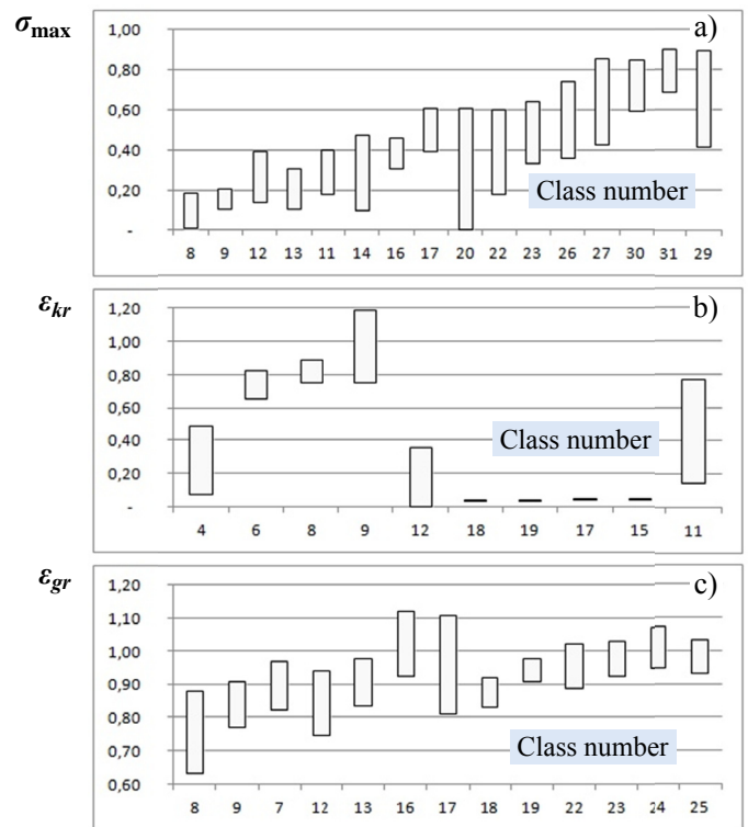
Fig. 10. Characteristics diagrams for final nodes in regression trees for variables: a) \sigma_{max} , b) \epsilon_{kr} , c) \epsilon_{gr}
