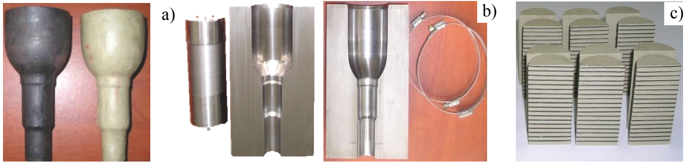
Fig. 2. a) Comparison of a forging made of steel after II extrusion operation with a forging made of filia wax, b) a tool set: a punch, two matrix halves, tightening belts, c) preforms made of modelling materials with horizontal flow lines
