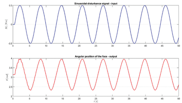
Fig. 3. Mathematical model response to a sinusoidal input.
