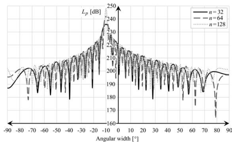
Fig. 17. Results of the acoustic field distribution calculations in the form of L_p(x) for y = 0 , z = R = 130 mm and the focus inclined by 10^\circ , for the number of activated transducers of the sector as follows: n = 32, 64 , and 128.
