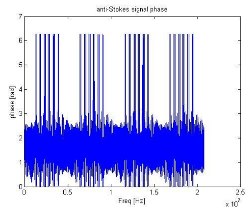
Fig. 16. Anti-Stokes signal phase for -5°C
