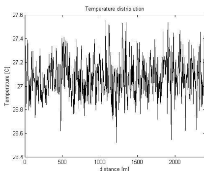
Fig. 18. Temperature variations due to the shot and thermal noise
