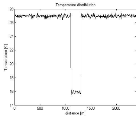
Fig. 15. Temperature profile for 16°C
