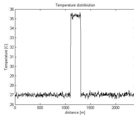
Fig. 9. Temperature profile for 35°C
