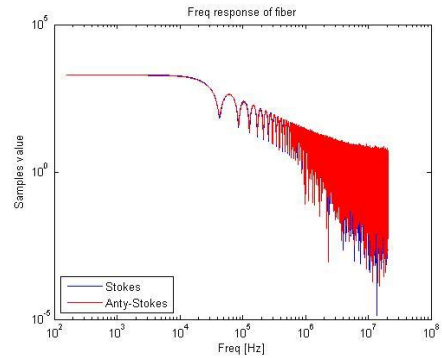
Fig. 7. Frequency response for 35°C
