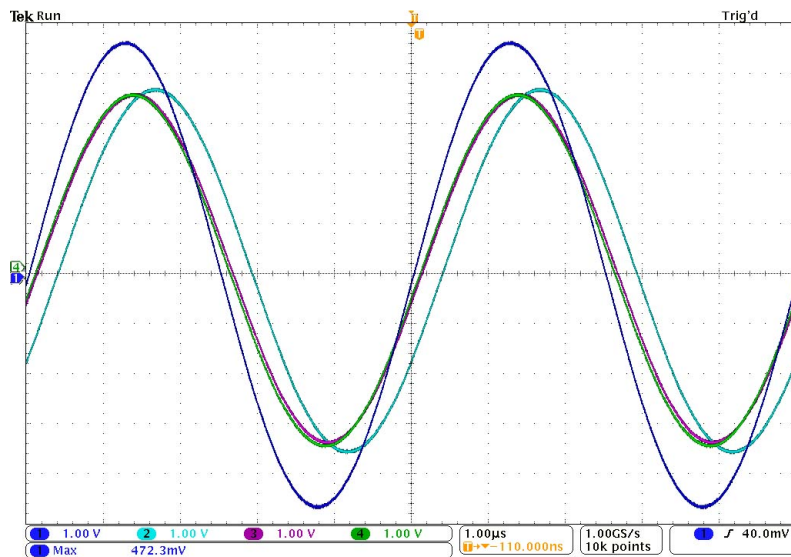
Fig. 5. Oscillograms of voltage waveforms at the ends of ignition cables supplied by sinusoidal voltage
