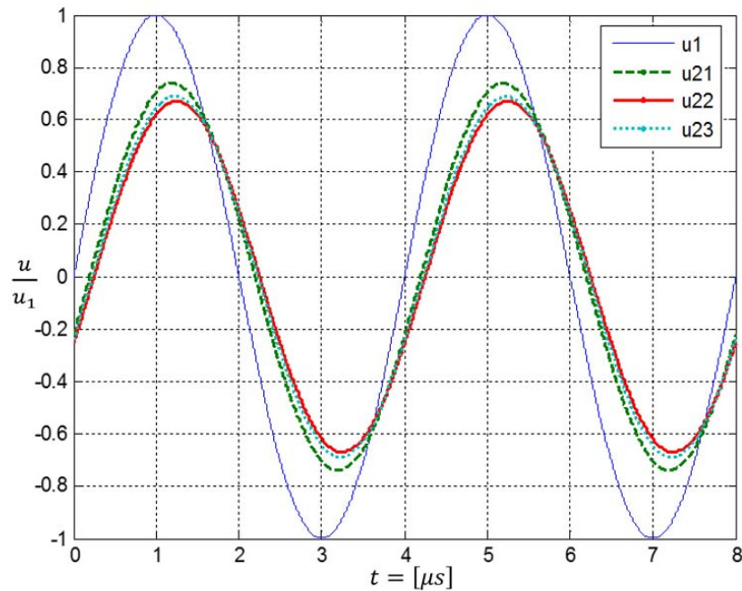
Fig. 3. Voltage at the end of the line for sinusoidal voltage at the input of the line
