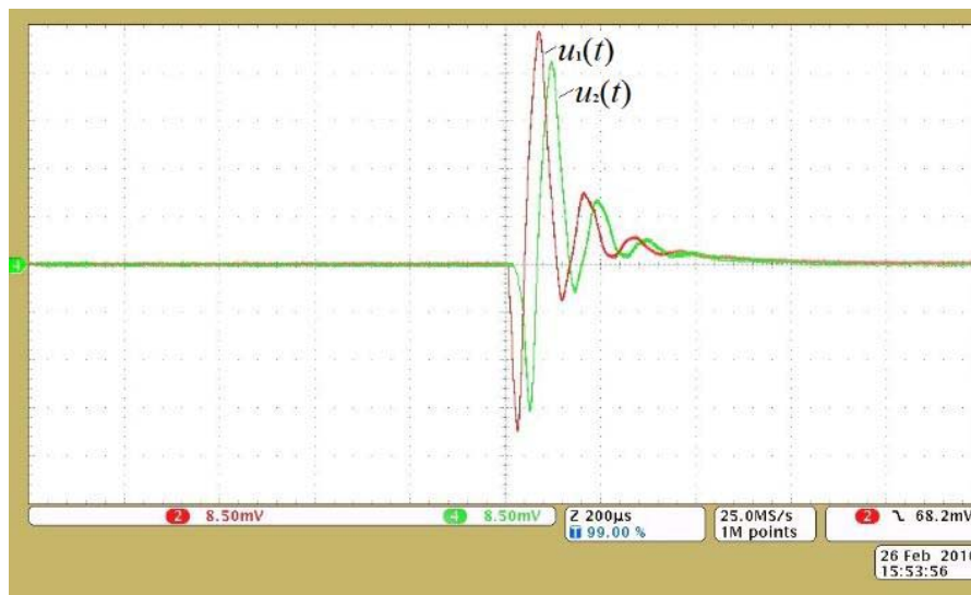
Fig. 2. The waveform of the secondary voltage of the ignition coil u_1(t) and the voltage at the end of the ignition cable u_2(t)
