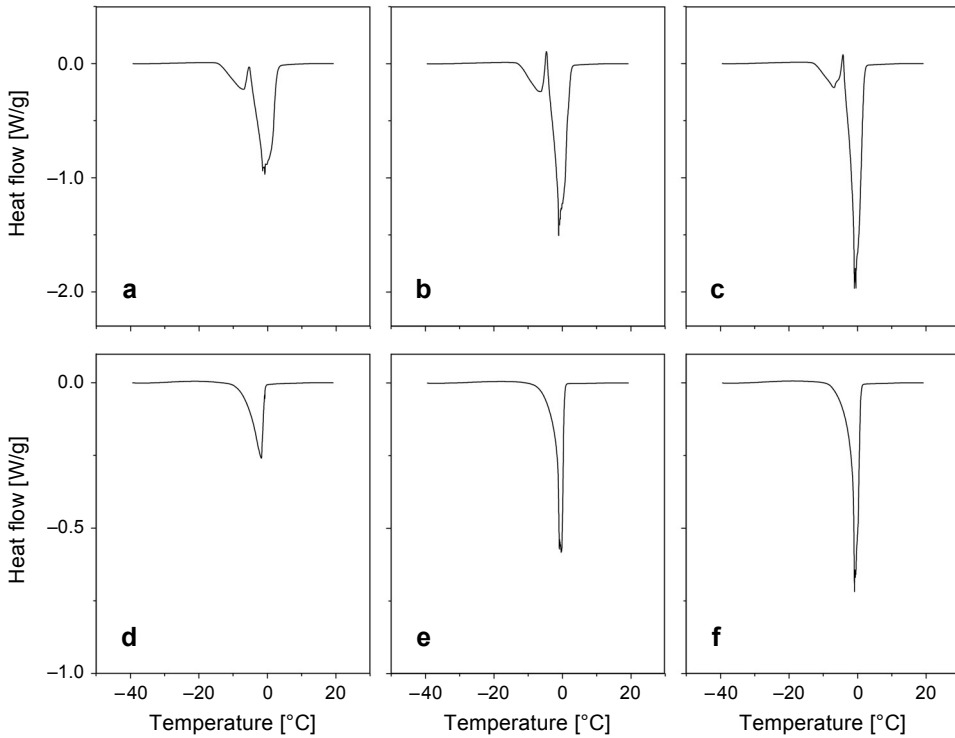
Fig. 5. Exemplary DSC melting endotherms for Proclear: control (a), 0.1% HA (b), 0.3% HA (c); Night & Day: control (d), 0.1% HA (e), 0.3% HA (f). Figures present heat flow in function of temperature where two peaks (Proclear) or one peak (Night & Day) were observed.
