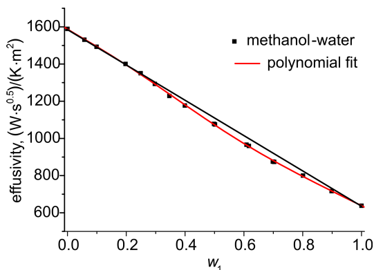
Fig. 2. Dependence of thermal effusivity, e , of aqueous methanol solution on the mass fraction w_1 of methanol at T = 25^\circ\text{C} , obtained by the photoacoustic method.
